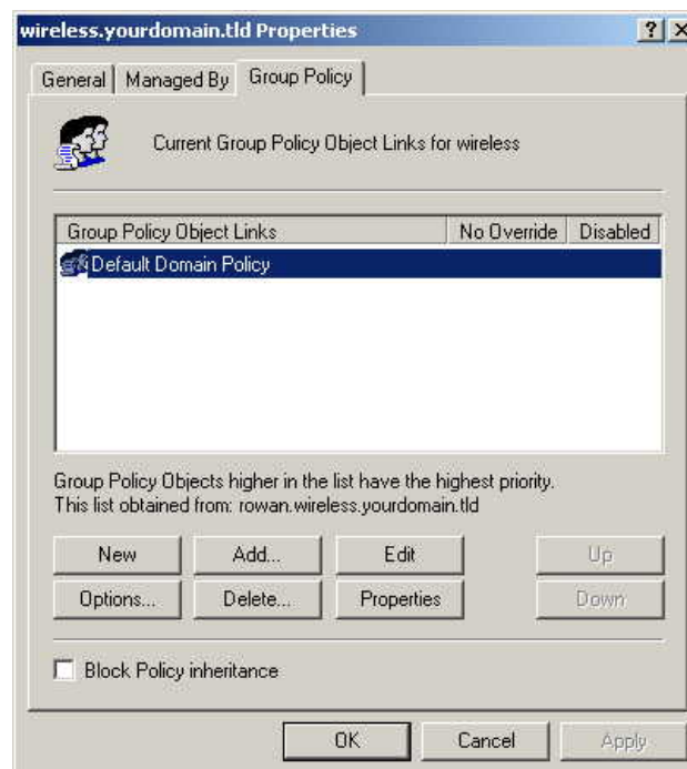
Figure 56: Group Policy Tab
