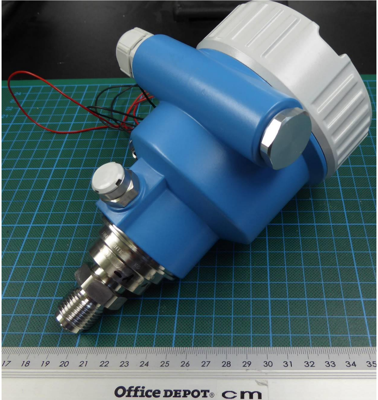
EUT VE113_A_03 in representative housing – 3D view 2
