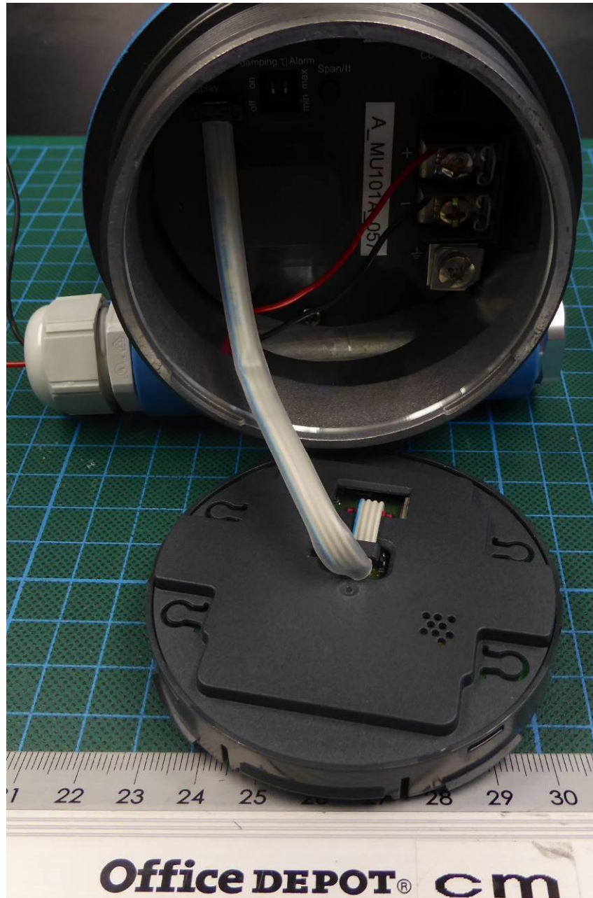
EUT VE113_A_03 in representative housing – housing open 2
