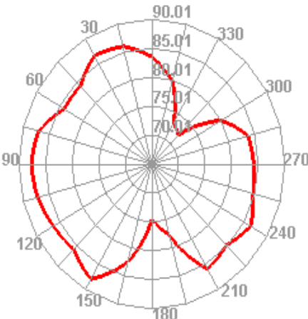
Bluetooth 39 TIS Phi=45
