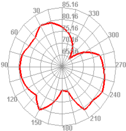
Bluetooth 78 TIS Phi=45
