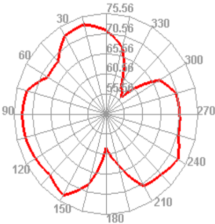
Bluetooth 0 TIS Phi=45
