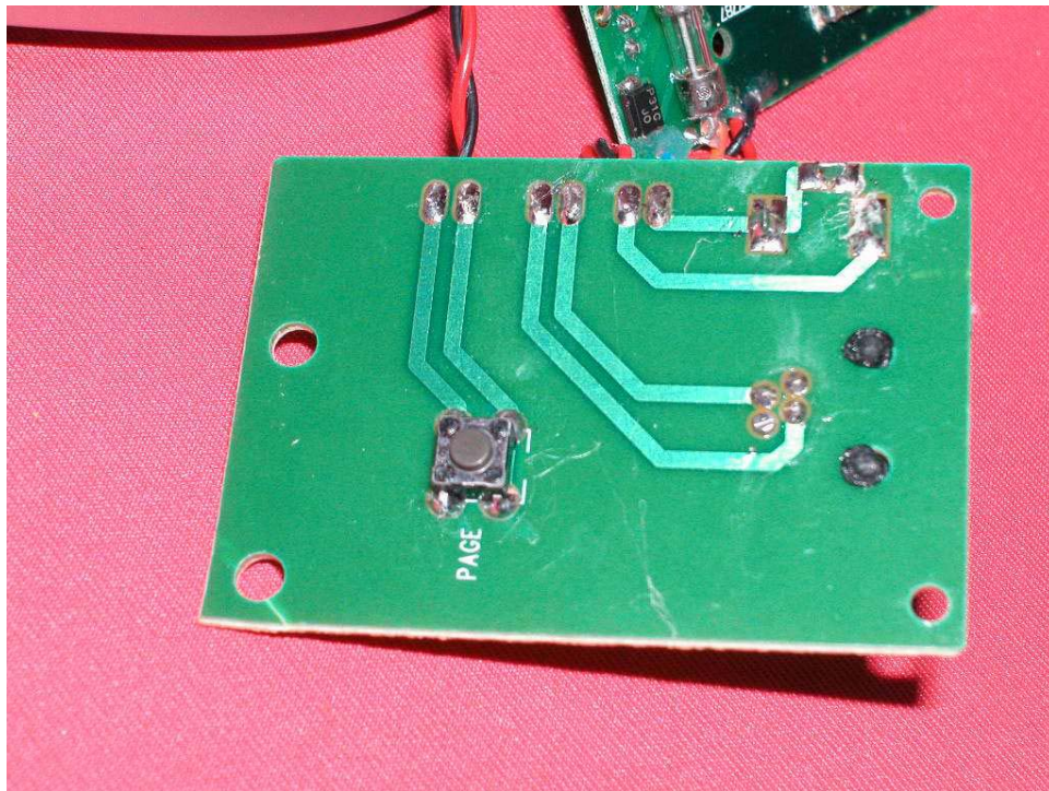
Base AC Jack and Telephone Line Jack PCB rear side
