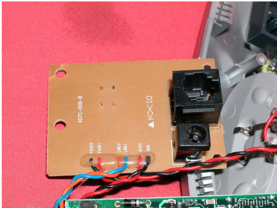
Base AC Jack and Telephone Line Jack PCB front side
