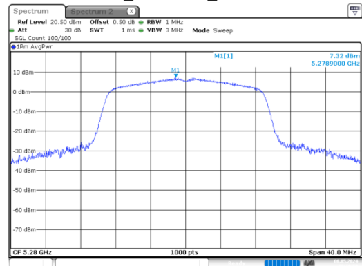
n20_5280MHz_Chain 1
