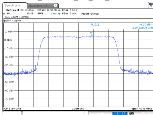
ax20_5240MHz_RU_Full_Chain 0
