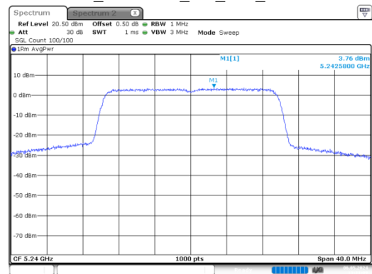
ax20_5240MHz_RU_Full_Chain 1
