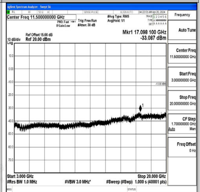
Band4_10MHz_16QAM_20000_1RB#0_3000~20000_3000~20000
