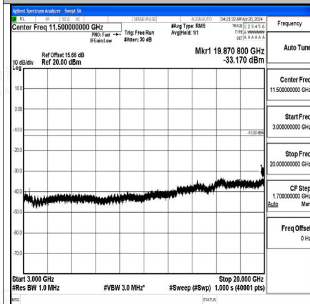
Band4_10MHz_QPSK_20000_1RB#0_3000~20000_300 0~20000
