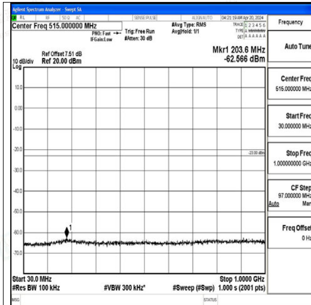
Band4_10MHz_QPSK_20000_1RB#0_30~1000_30~100 0
