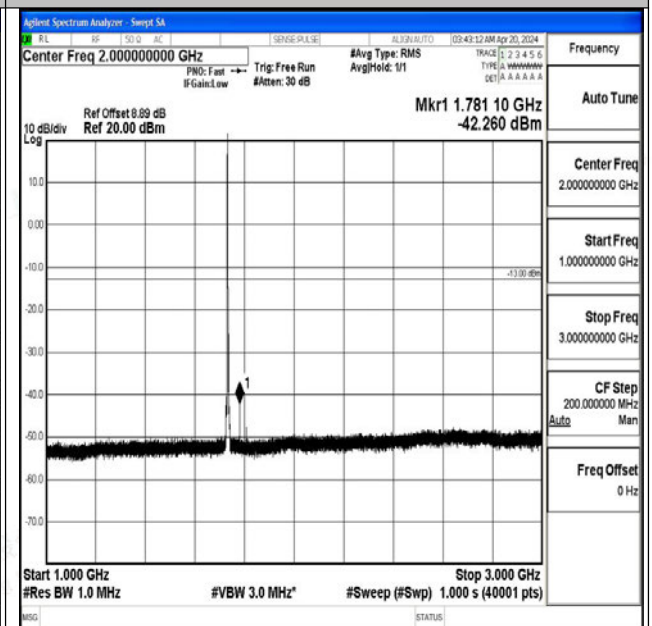
Band4_3MHz_QPSK_20175_1RB#0_1000~3000_1000~3000
