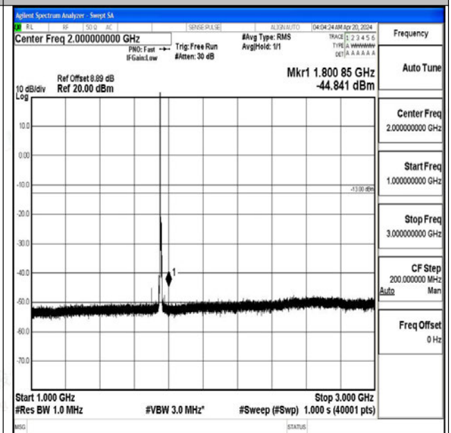
Band4_5MHz_QPSK_20375_1RB#0_1000~3000_1000~3000
