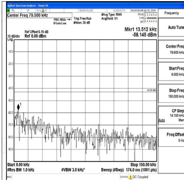
Band4_5MHz_QPSK_20375_1RB#0_0.009~0.15_0.009~0.15
