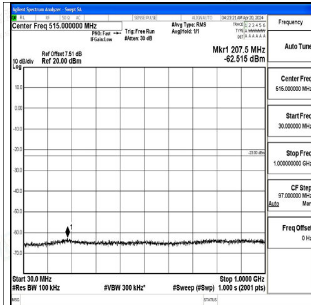
Band4_10MHz_QPSK_20350_1RB#0_30~1000_30~1000 0
