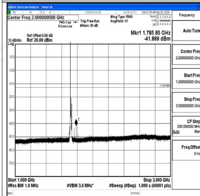
Band4_10MHz_16QAM_20000_1RB#0_1000~3000_1000~3000
