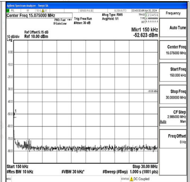
Band4_3MHz_QPSK_20175_1RB#0_0.15~30_0.15~30
