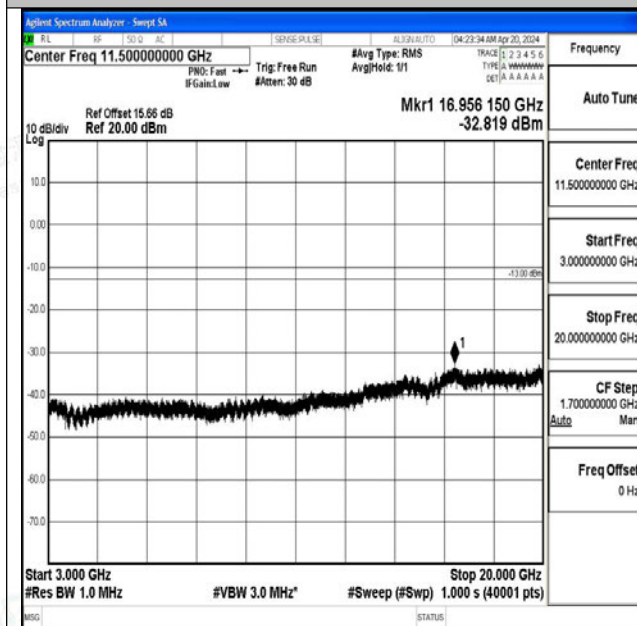
Band4_10MHz_QPSK_20350_1RB#0_3000~20000_300 0~20000
