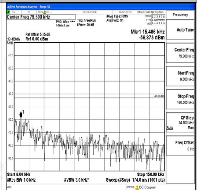
Band4_10MHz_16QAM_20350_1RB#0_0.009~0.15_0.0 09~0.15
