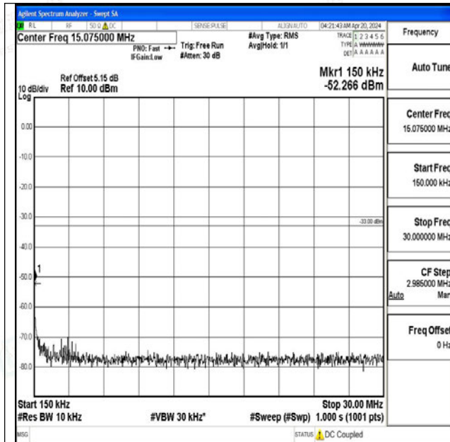
Band4_10MHz_16QAM_20000_1RB#0_0.15~30_0.15~3
