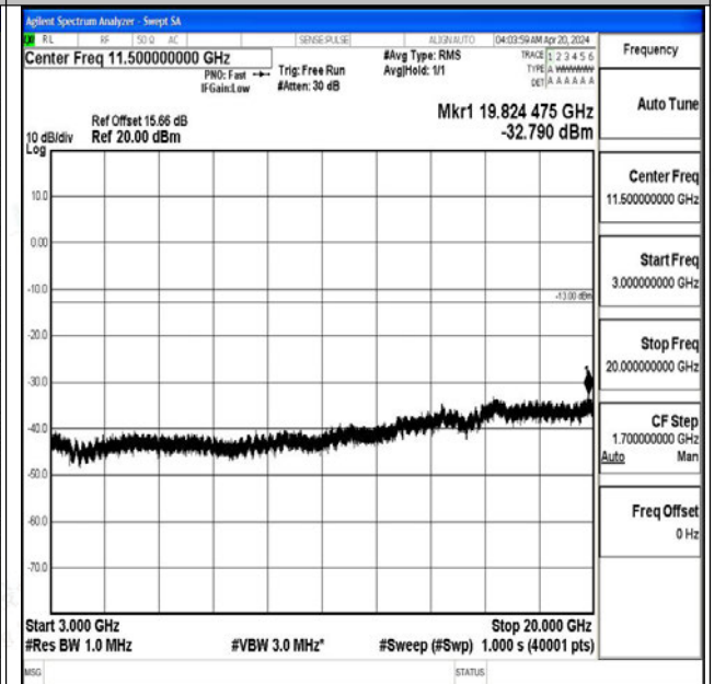
Band4_5MHz_16QAM_20175_1RB#0_3000~20000_3000 0~20000
