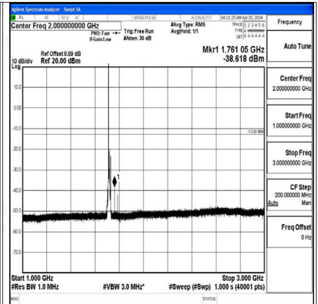
Band4_10MHz_QPSK_20000_1RB#0_1000~3000_1000 ~3000
