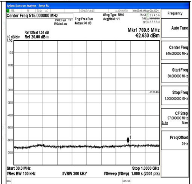
Band4_5MHz_16QAM_20175_1RB#0_30~1000_30~1000 0
