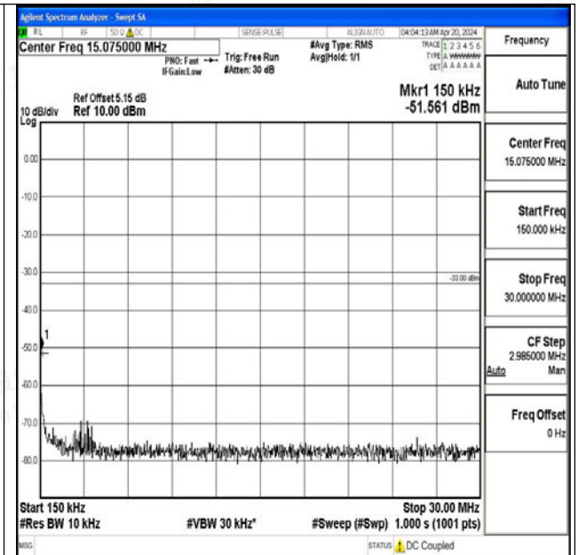
Band4_5MHz_QPSK_20375_1RB#0_0.15~30_0.15~30
