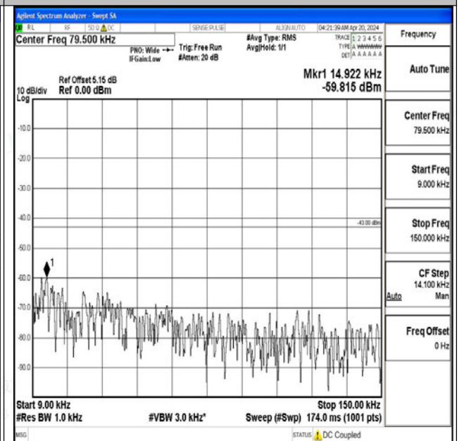
Band4_10MHz_16QAM_20000_1RB#0_0.009~0.15_0.0 09~0.15
