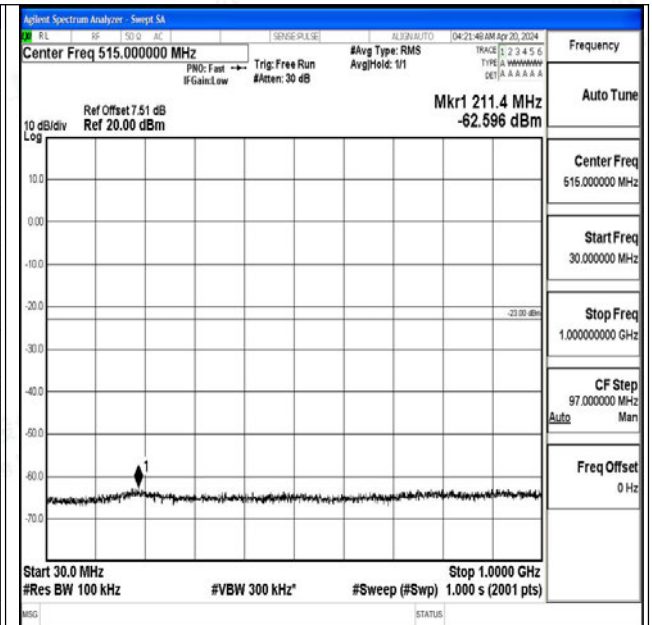
Band4_10MHz_16QAM_20000_1RB#0_30~1000_30~10
