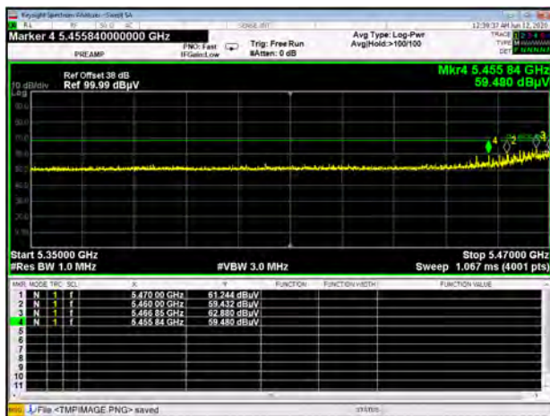
Band III 11ac20 CH100 Peak
