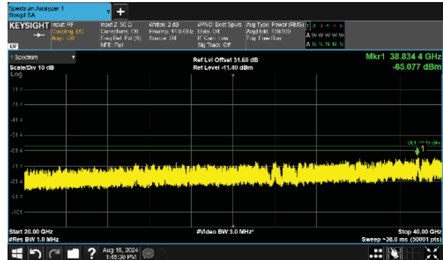
Port 1 20 MHz Channel Bandwidth QPSK Modulation Mid Channel, 3500.01 MHz
