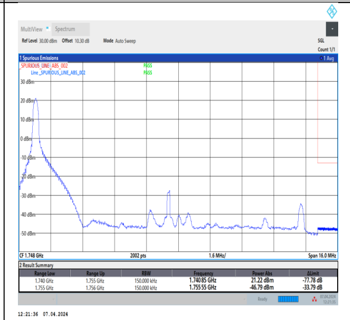
Band4_15MHz_64QAM_20325_1RB#0
