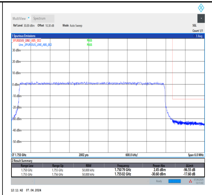
Band4_5MHz_64QAM_20375_25RB#0
