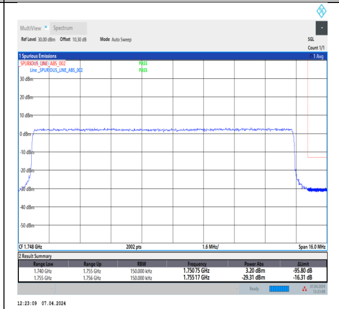
Band4_15MHz_16QAM_20325_75RB#0
