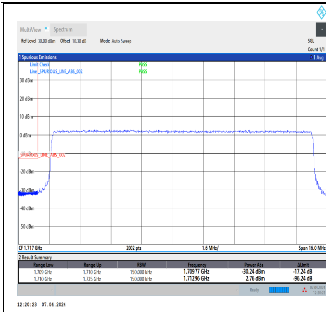
Band4_15MHz_16QAM_20025_75RB#0
