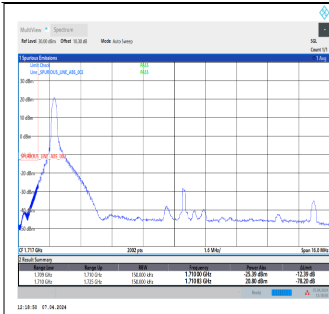
Band4_15MHz_64QAM_20025_1RB#0
