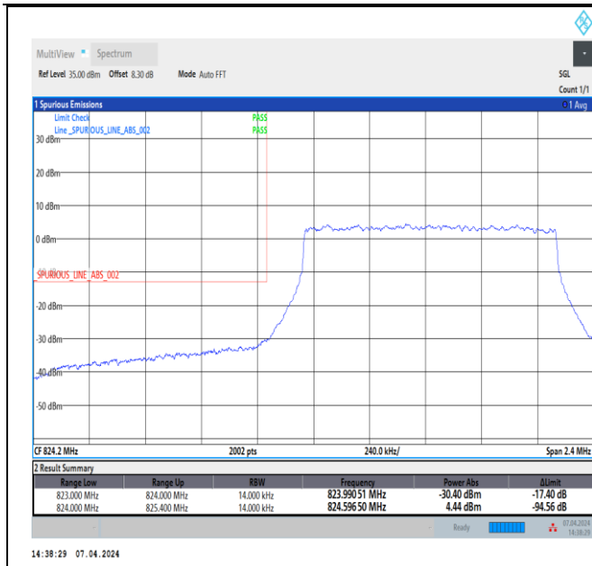
Band5_1.4MHz_16QAM_20407_6RB#0
