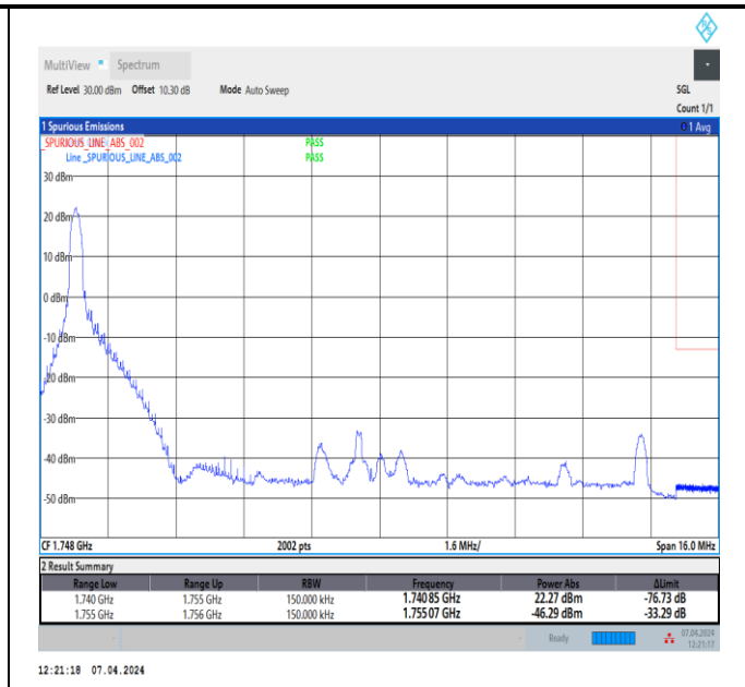
Band4_15MHz_16QAM_20325_1RB#0
