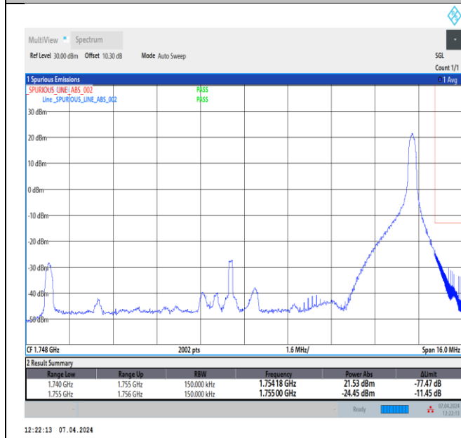
Band4_15MHz_16QAM_20325_1RB#74
