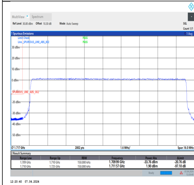
Band4_15MHz_64QAM_20025_75RB#0
