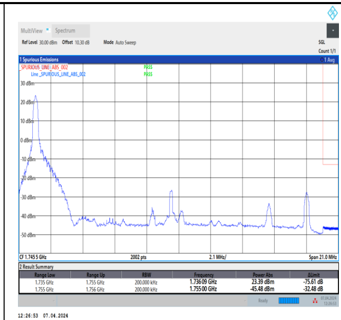
Band4_20MHz_QPSK_20300_1RB#0
