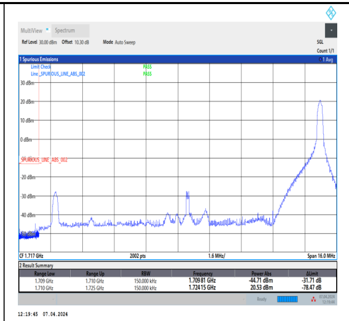
Band4_15MHz_64QAM_20025_1RB#74
