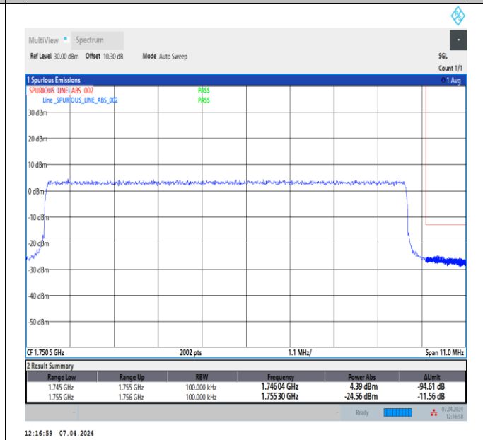
Band4_10MHz_QPSK_20350_50RB#0
