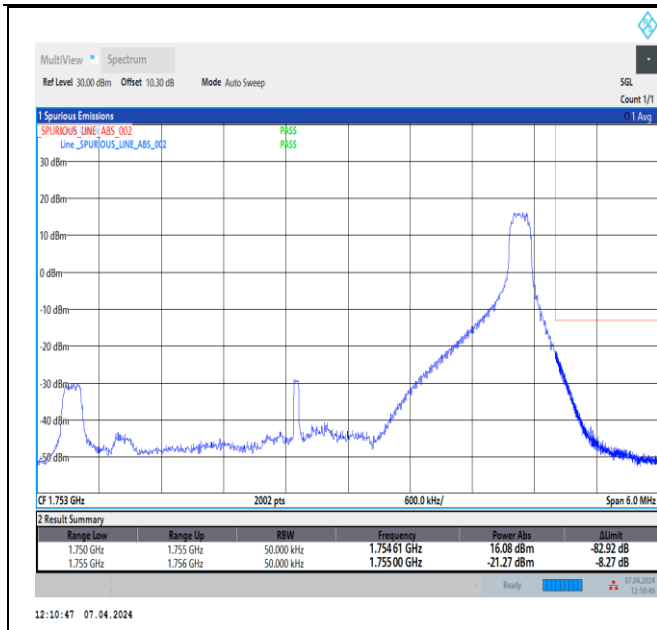
Band4_5MHz_64QAM_20375_1RB#24
