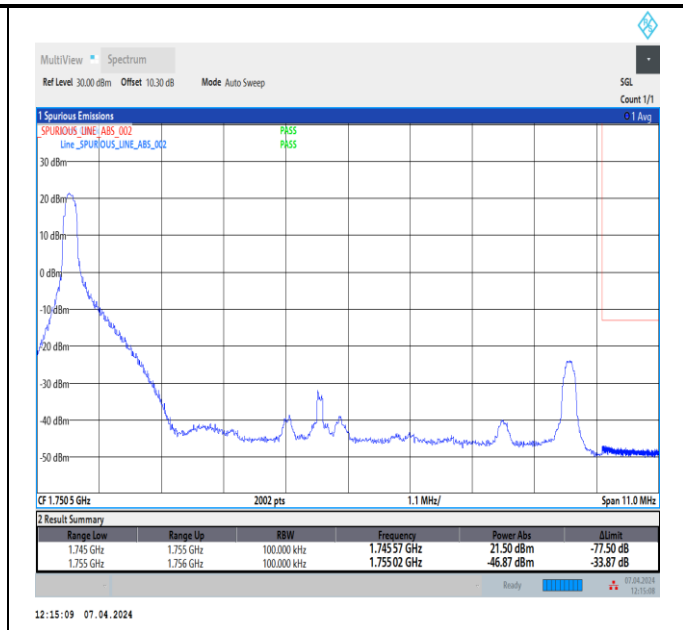
Band4_10MHz_QPSK_20350_1RB#0
