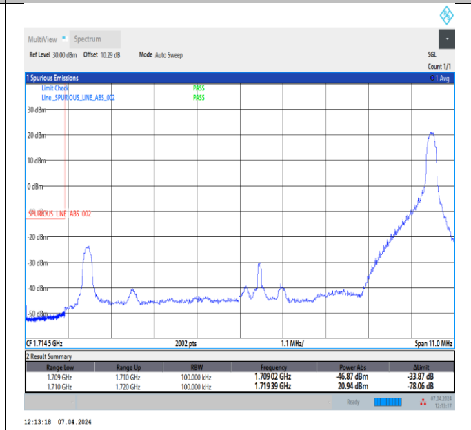
Band4_10MHz_QPSK_20000_1RB#49
