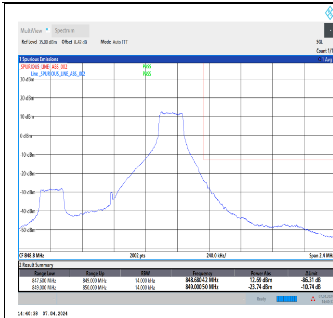
Band5_1.4MHz_64QAM_20643_1RB#5
