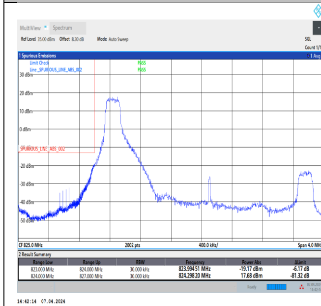
Band5_3MHz_QPSK_20415_1RB#0
