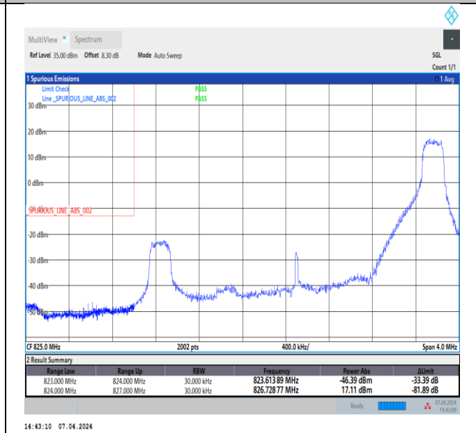
Band5_3MHz_QPSK_20415_1RB#14
