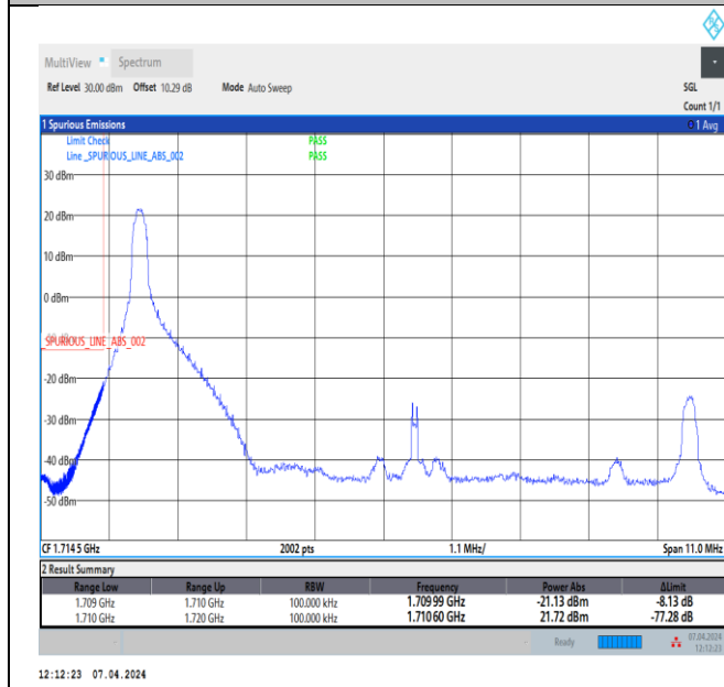
Band4_10MHz_QPSK_20000_1RB#0
