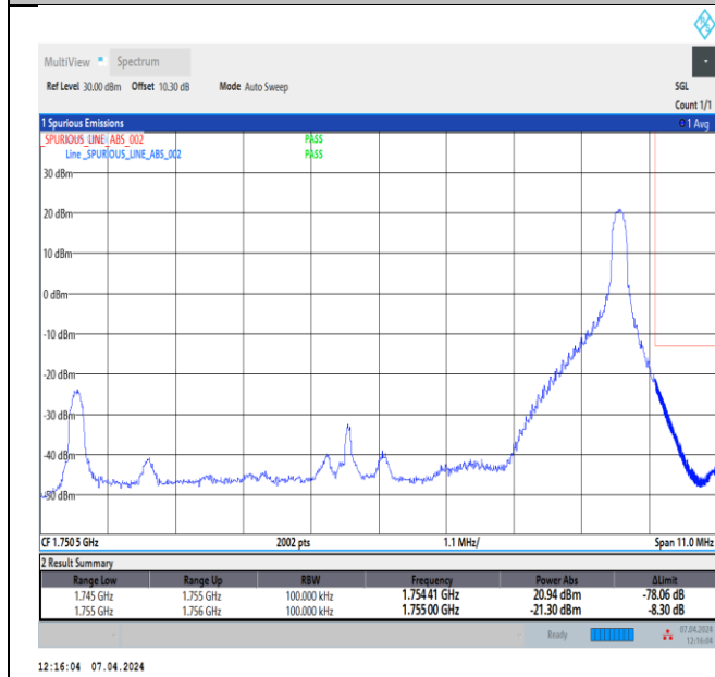
Band4_10MHz_QPSK_20350_1RB#49
