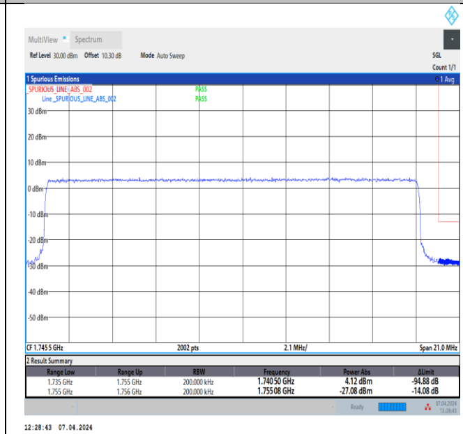
Band4_20MHz_QPSK_20300_100RB#0
