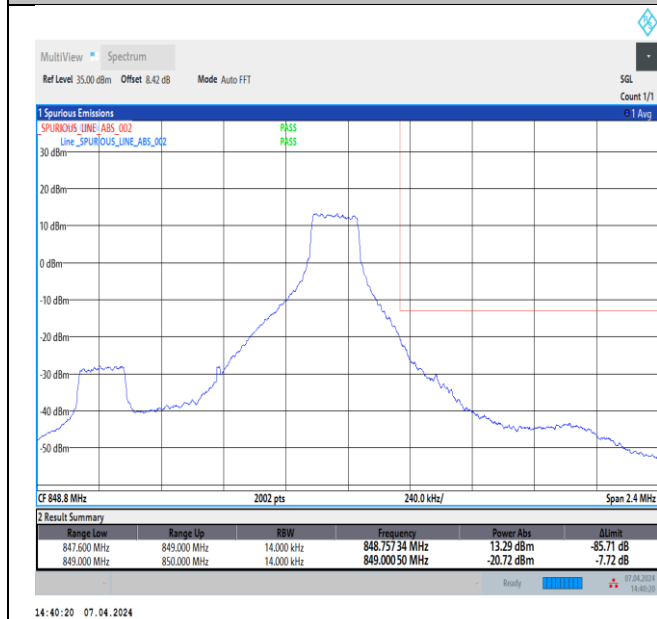
Band5_1.4MHz_16QAM_20643_1RB#5
