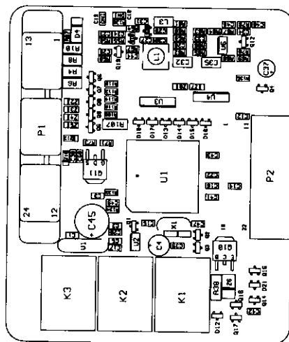
ASSEMBLY TOP
