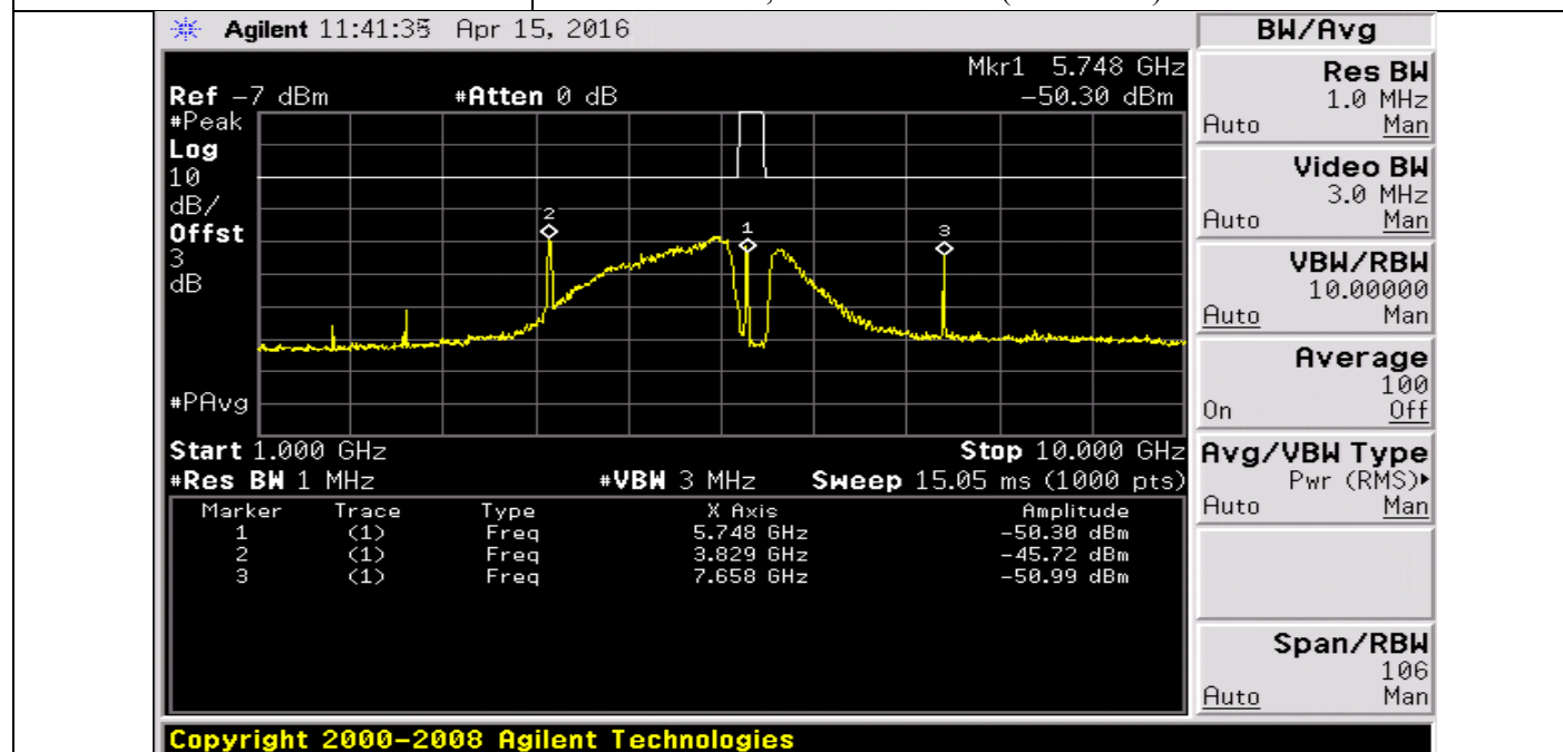
Title: TX Spurious Emissions from 1GHz-10GHz – Ch149 (5745 MHz)
