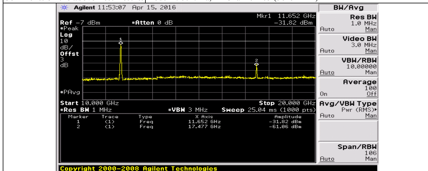
Title: TX Spurious Emissions from 10GHz-20GHz – Ch165 (5825 MHz)
