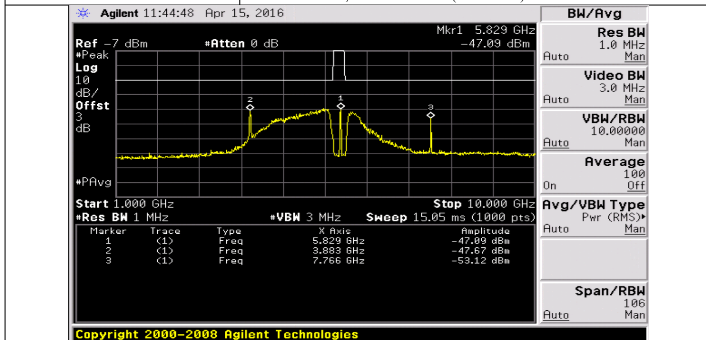
Title: TX Spurious Emissions from 1GHz-10GHz – Ch165 (5825 MHz)
