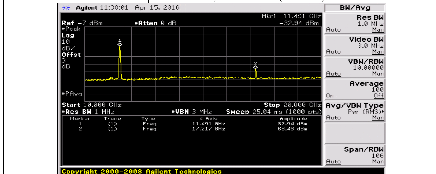
Title: TX Spurious Emissions from 10GHz-20GHz – Ch149 (5745 MHz)
