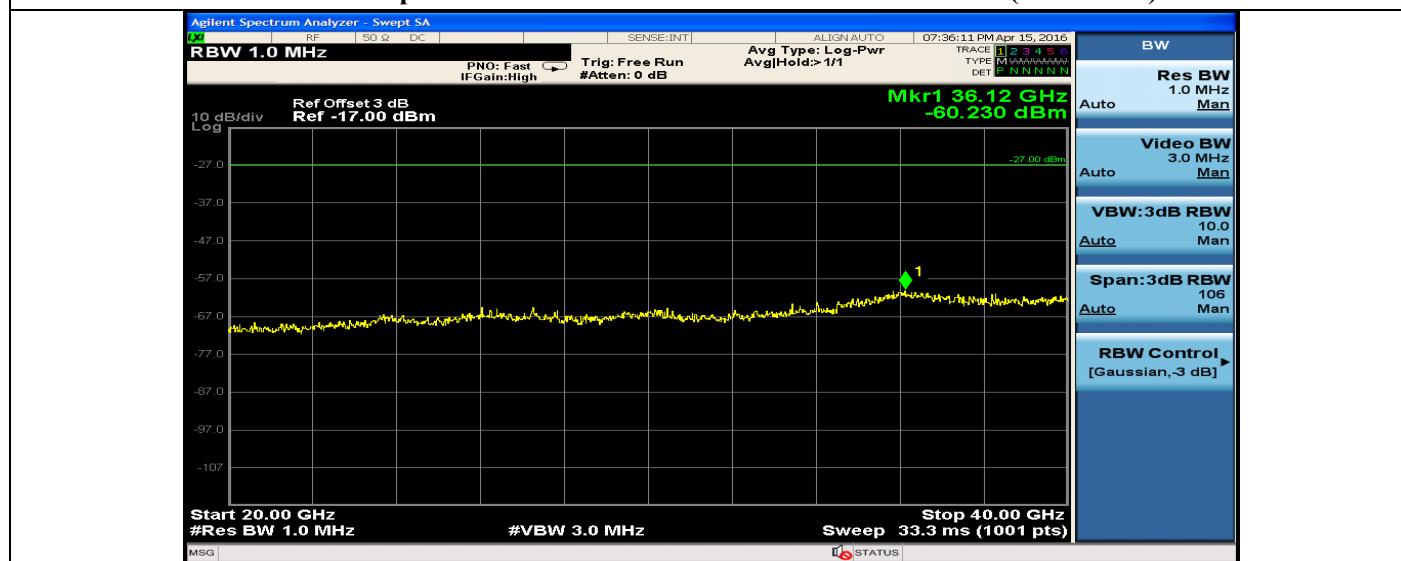
Title: TX Spurious Emissions from 20GHz-40GHz – Ch165 (5825 MHz)
