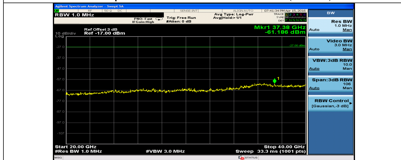
Title: TX Spurious Emissions from 20GHz-40GHz – Ch149 (5745 MHz)
