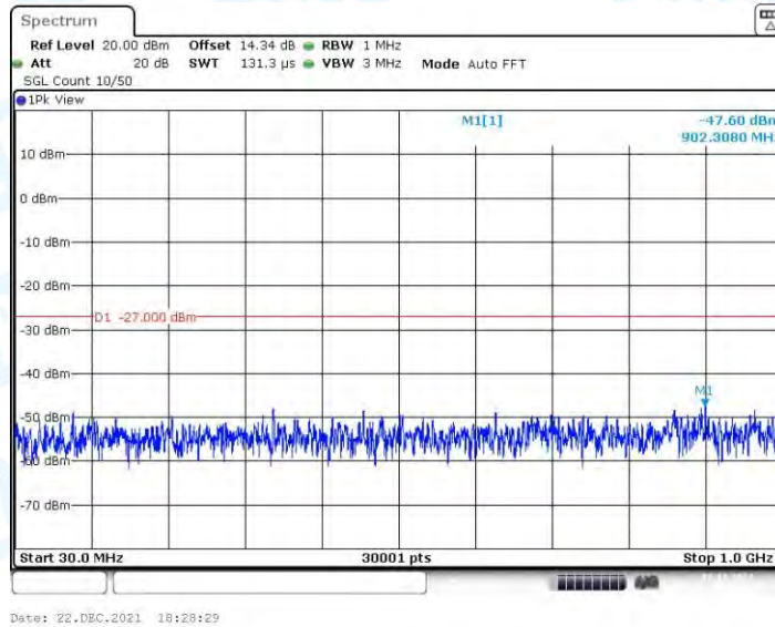
11A_Ant3_5700_30~1000
