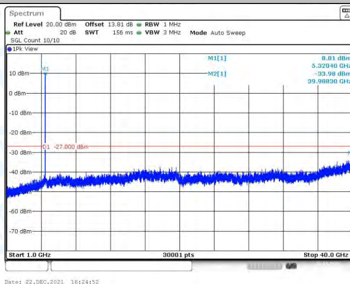
11A_Ant3_5320_1000~40000
