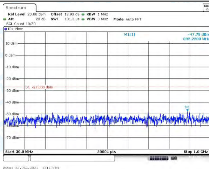
11A_Ant3_5300_30~1000
