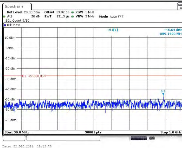
11A_Ant1_5785_30~1000
