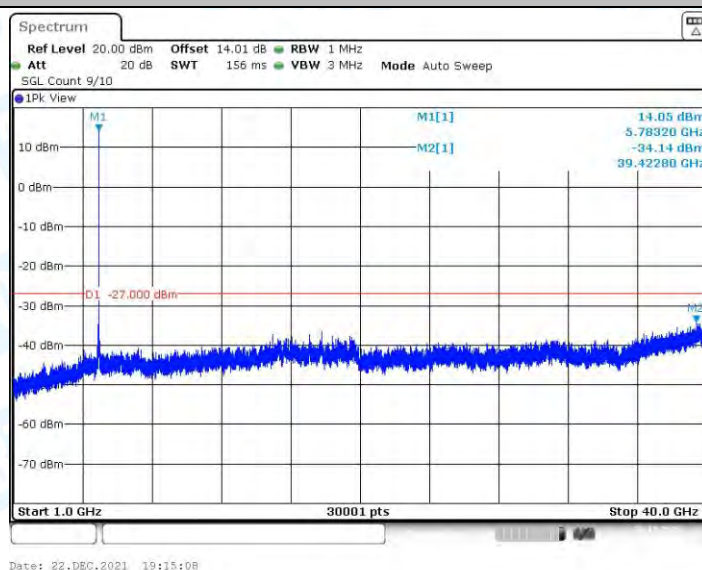
11A_Ant2_5785_1000~40000
