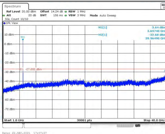
11A_Ant2_5700_1000~40000
