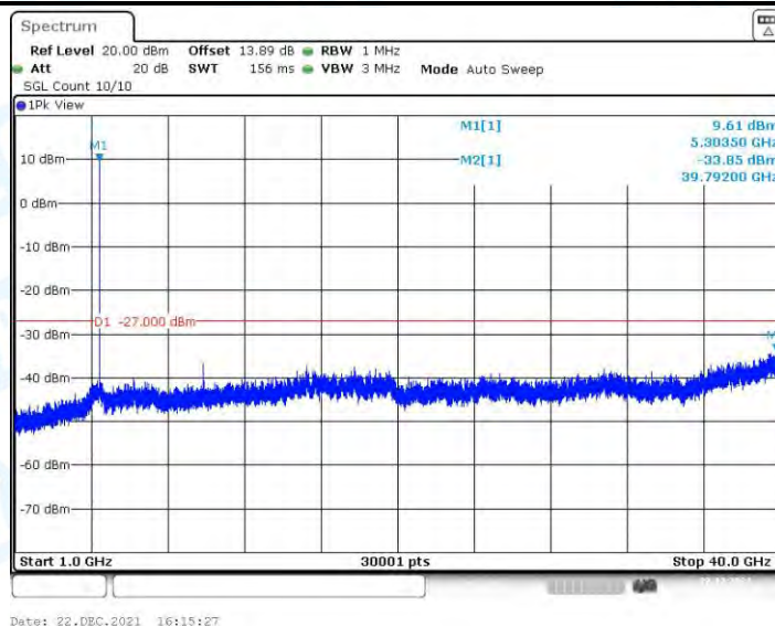
11A_Ant2_5300_1000~40000
