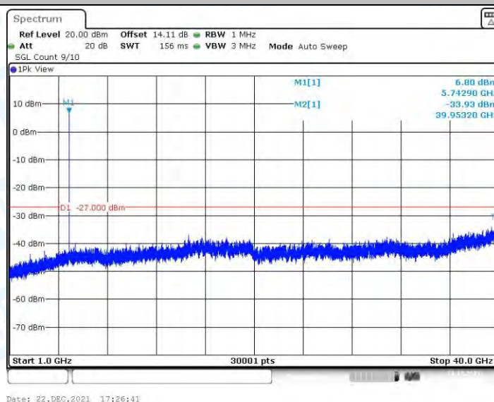
11A_Ant2_5745_1000~40000
