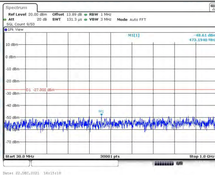
11A_Ant2_5300_30~1000
