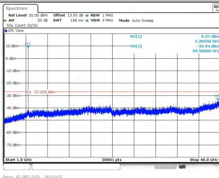
11A_Ant3_5300_1000~40000
