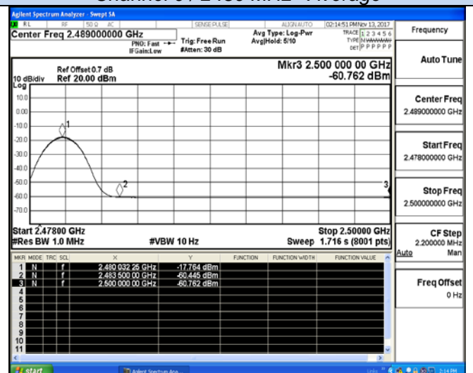
Channel 78 / 2480 MHz –Average
