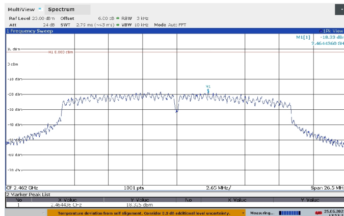
Figure 8(b): Power Spectral Density Plots.
