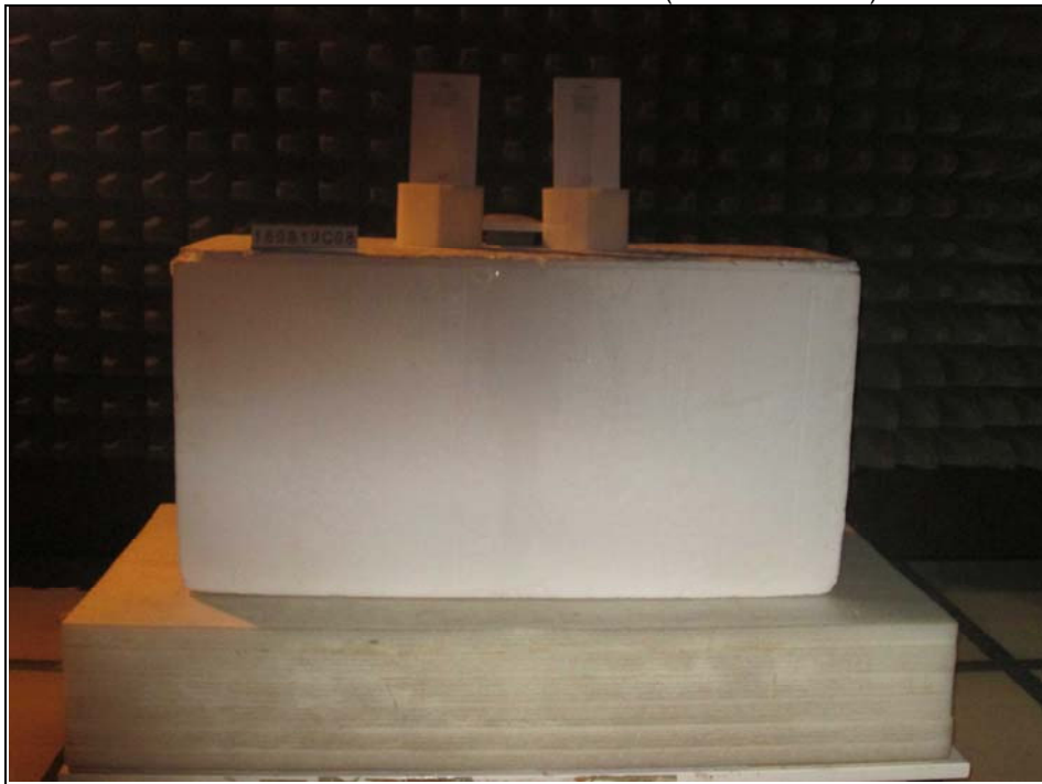
Radiated Emission Test above 1GHz (WLAN mode D)
