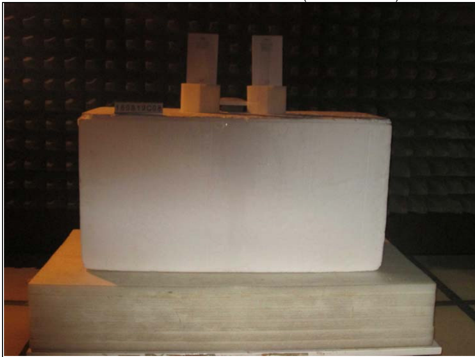
Radiated Emission Test above 1GHz (WLAN mode B)
