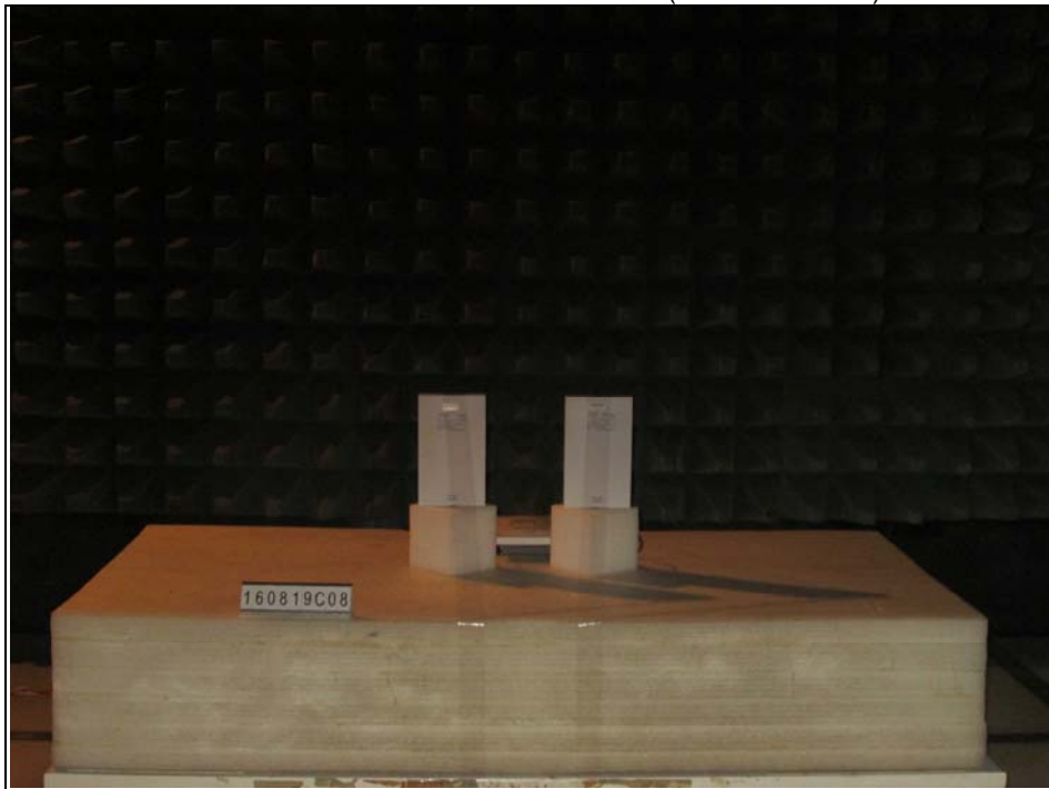
Radiated Emission Test below 1GHz (WLAN mode B)
