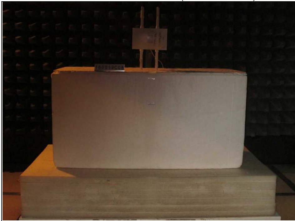
Radiated Emission Test above 1GHz (WLAN mode A & F)
