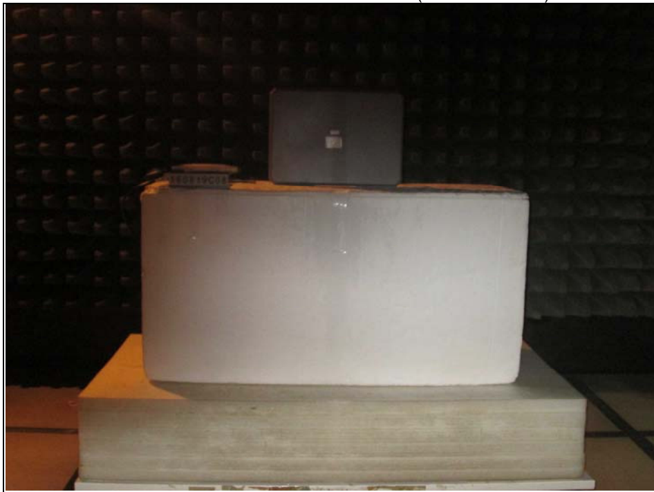
Radiated Emission Test above 1GHz (WLAN mode E)
