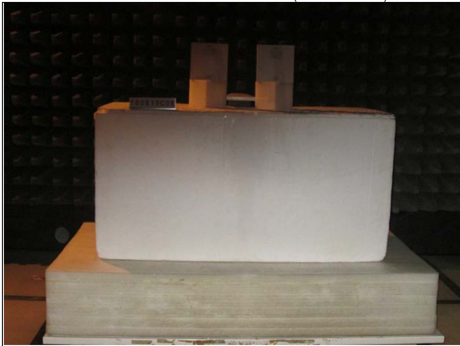
Radiated Emission Test above 1GHz (WLAN mode C)
