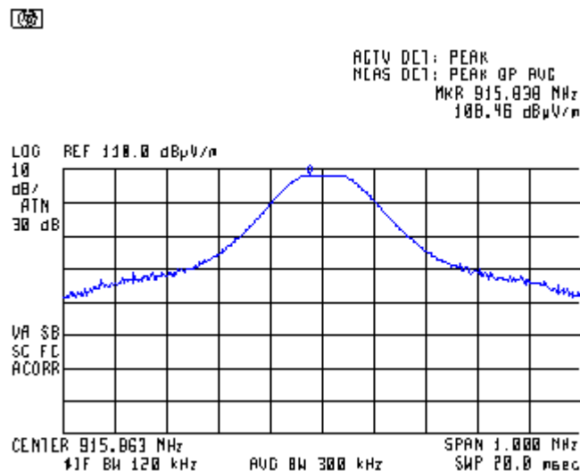
Plot 7.1.2 Field strength of carrier at mid frequency and Unom
