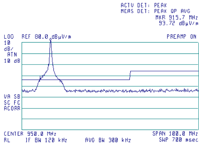
Plot 7.3.45 Radiated emission measurements from 900 to 1000 MHz at the high carrier frequency
