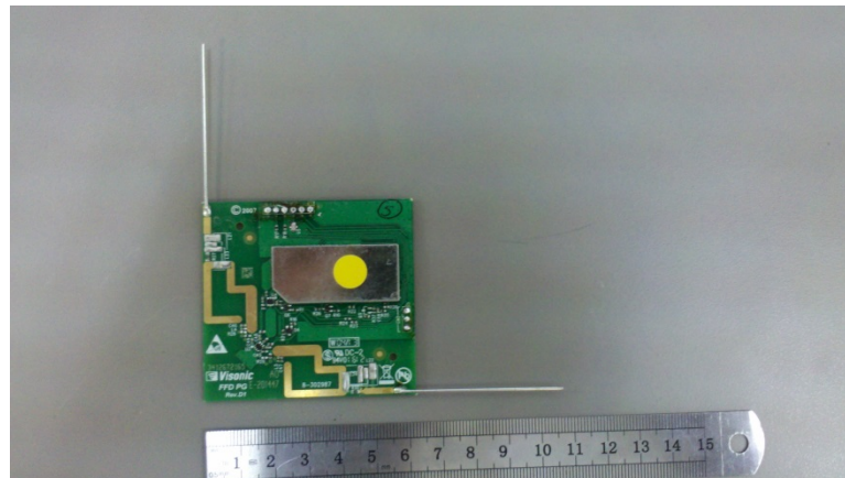
Photograph 7.4.1 Antenna assembly
