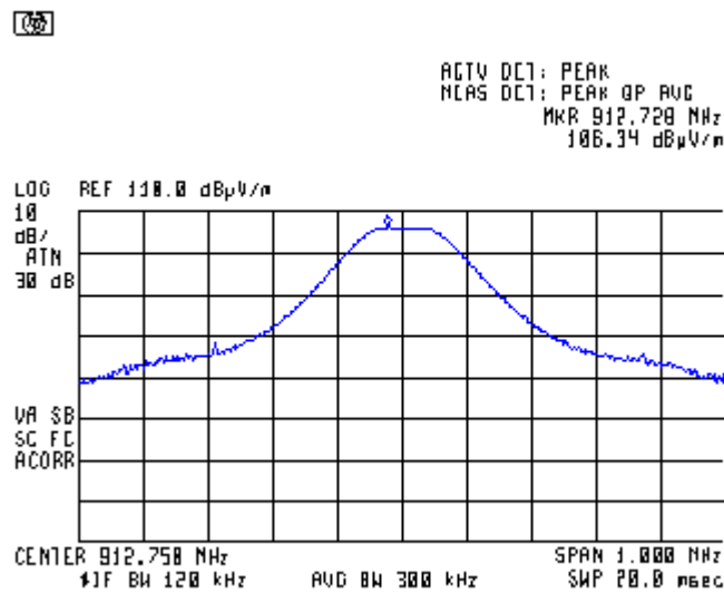
Plot 7.1.1 Field strength of carrier at low frequency and Unom
