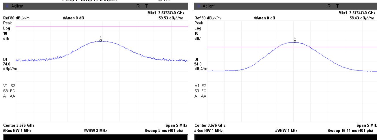
Plot 7.3.58 Radiated emission measurements at the fifth harmonic of low carrier frequency
