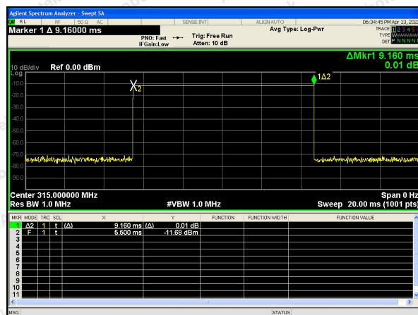
315MHz(ASK)-T period-20ms
