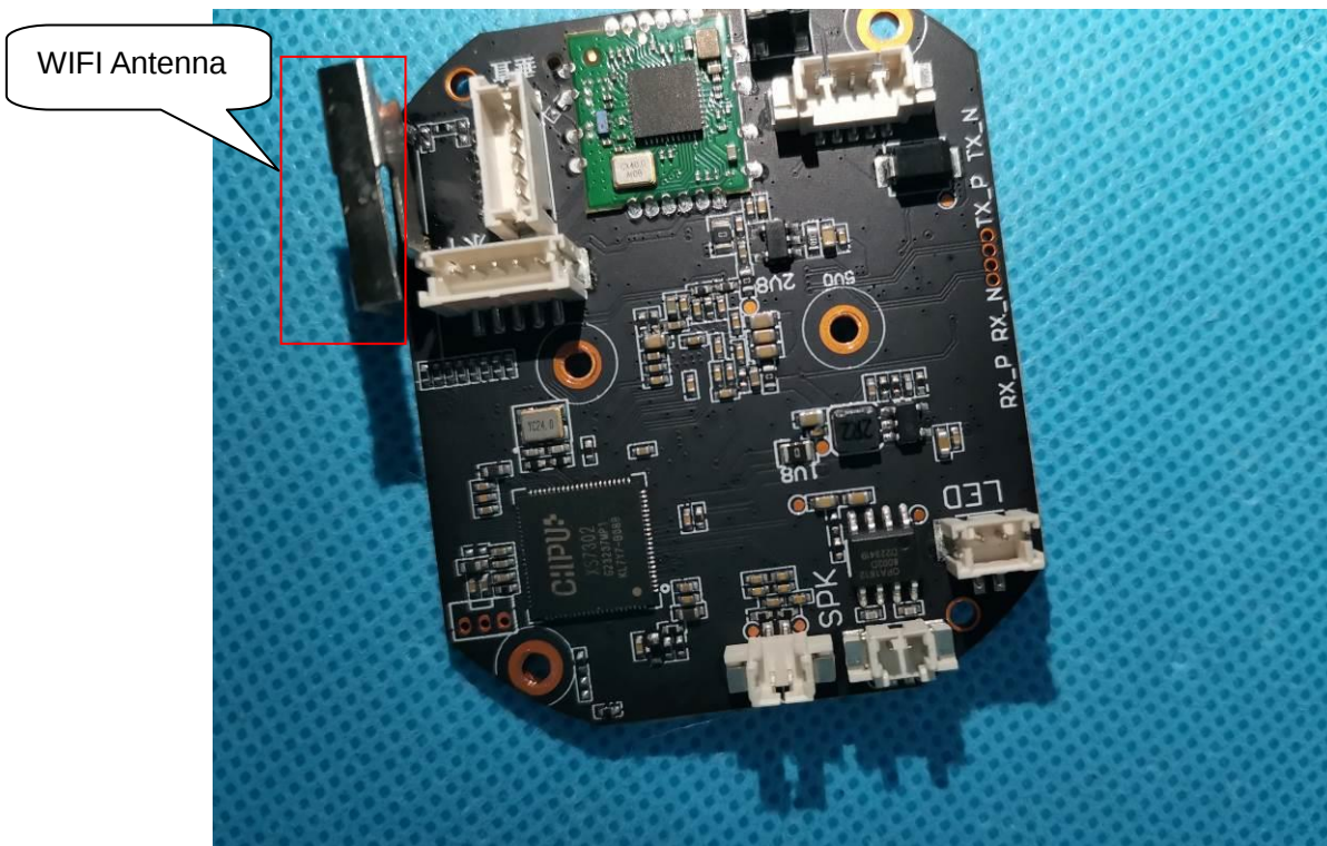
INTERNAL VIEW OF EUT (FIGURE 10)
