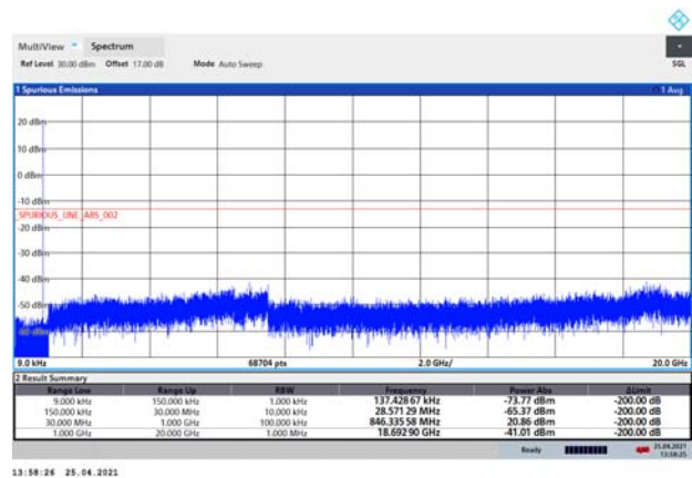
LTE-M Band 5 3MHz CH-High 9kHz~20GHz
