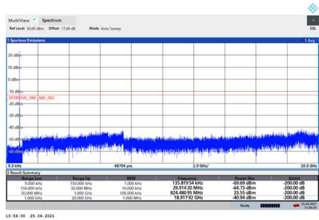
LTE-M Band 5 3MHz CH-Middle 9kHz~20GHz
