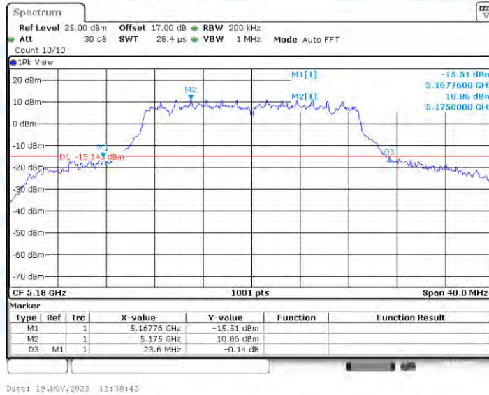
11N20-CDD_Ant4_5180
