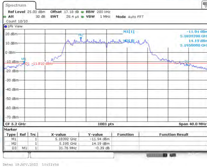
11A_Ant4_5200
