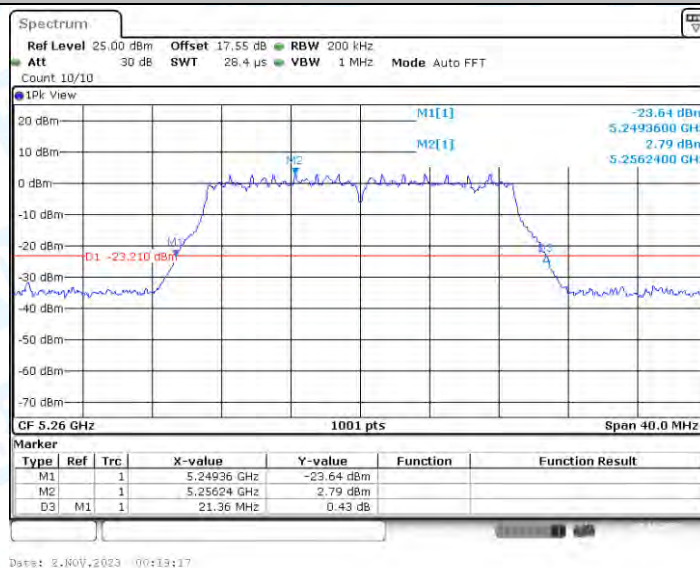
11A-CDD_Ant3_5260
