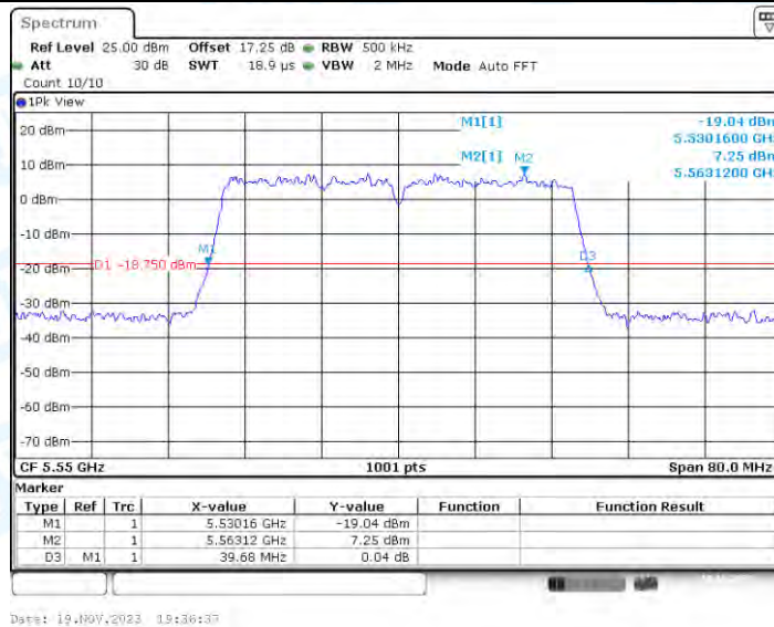
11N40-CDD_Ant4_5550
