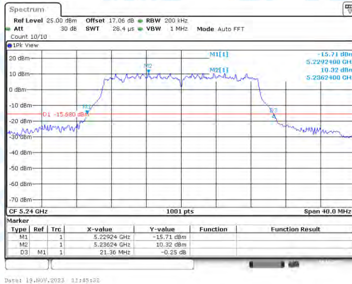
11AC20-CDD_Ant3_5240
