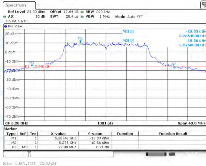
11A_Ant4_5280
