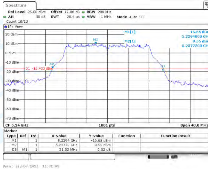
11A-CDD_Ant3_5240
