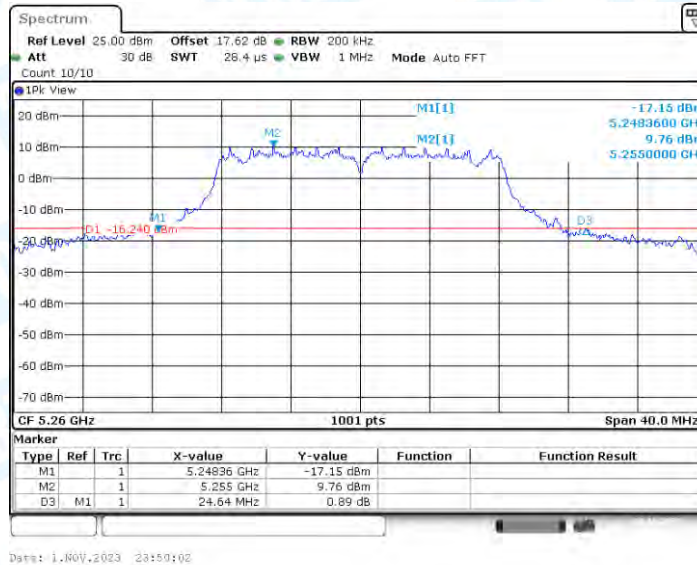
11A_Ant4_5260
