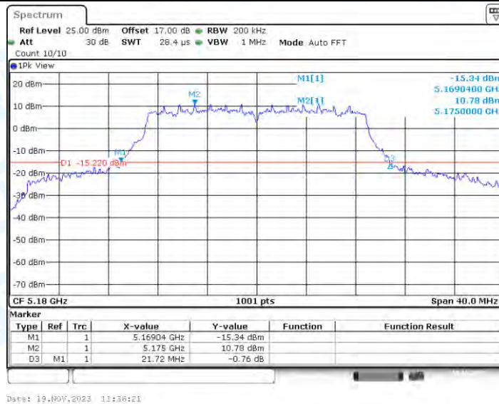
11AC20-CDD_Ant4_5180
