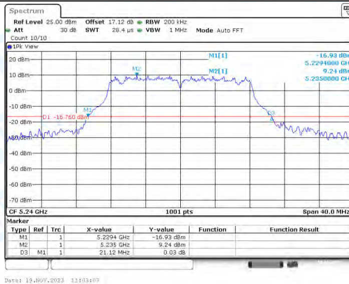
11A-CDD_Ant4_5240
