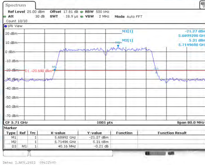
11N40-CDD_Ant4_5710
