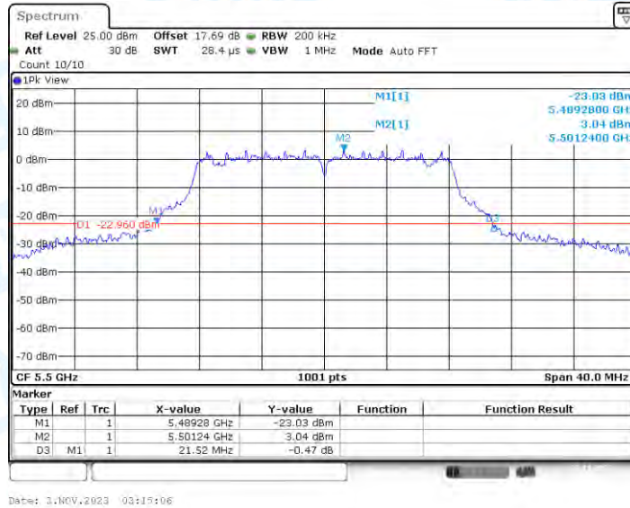
11A-CDD_Ant4_5500
