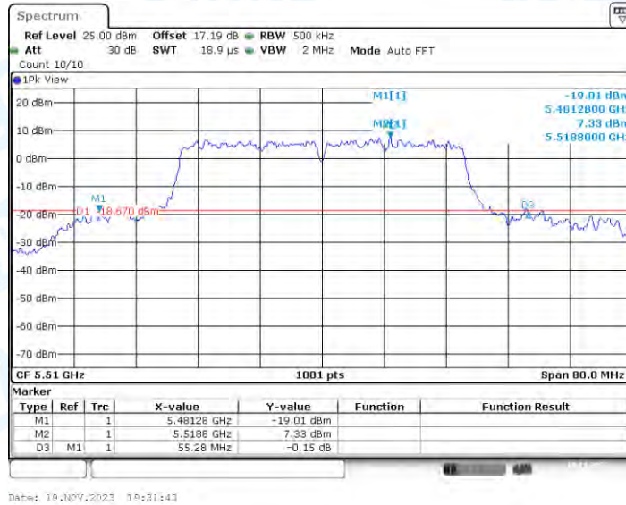
11N40-CDD_Ant4_5510
