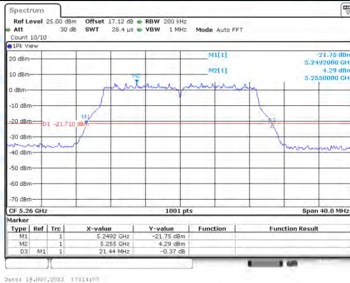
11AC20-CDD_Ant4_5260
