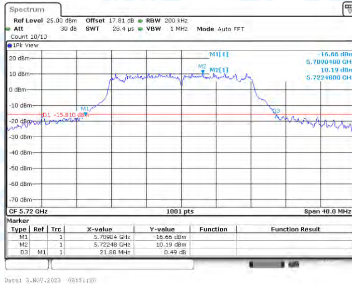
11A_Ant4_5720
