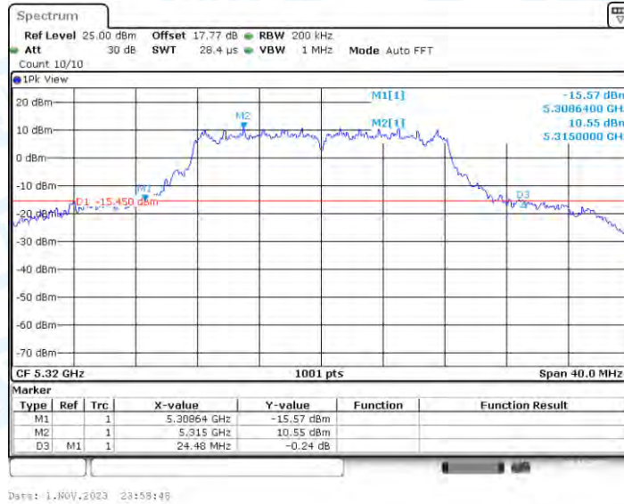
11A_Ant4_5320
