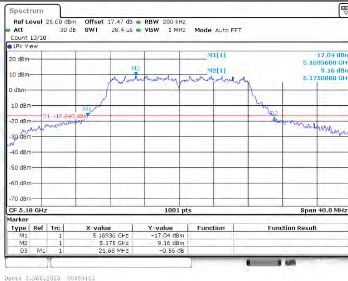
11A-CDD_Ant3_5180
