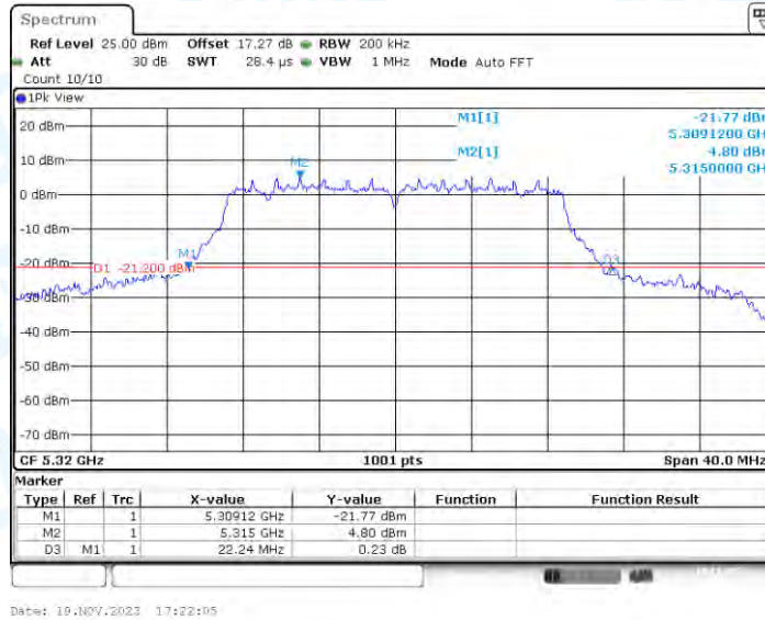
11AC20-CDD_Ant4_5320
