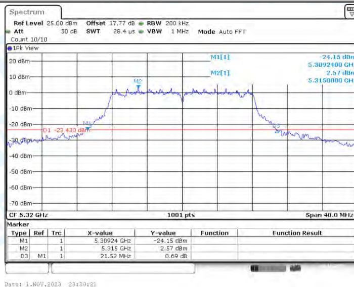
11A-CDD_Ant4_5320
