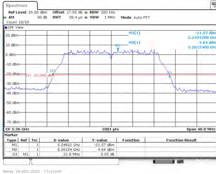
11AC20-CDD_Ant3_5260
