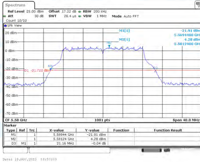
11A-CDD_Ant4_5580
