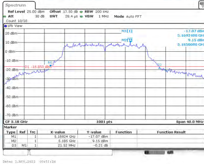
11A-CDD_Ant4_5180
