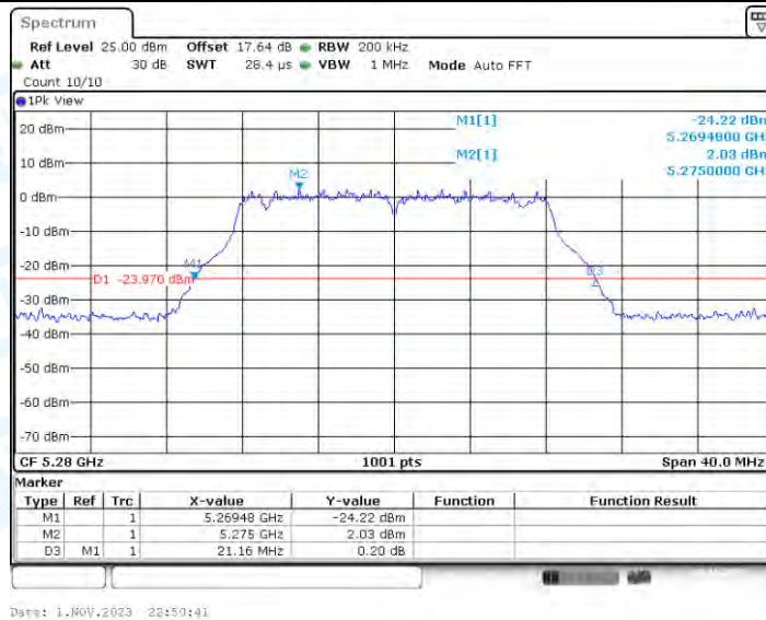
11A-CDD_Ant4_5280
