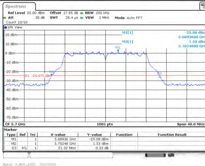
11A-CDD_Ant4_5700
