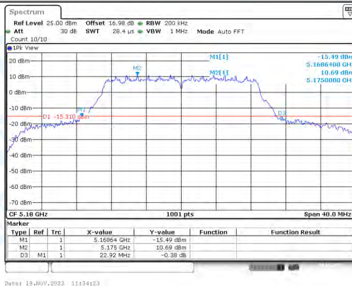
11AC20-CDD_Ant2_5180
