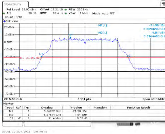
11A-CDD_Ant3_5580
