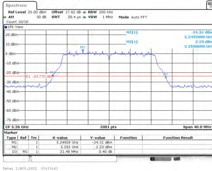
11A-CDD_Ant4_5260
