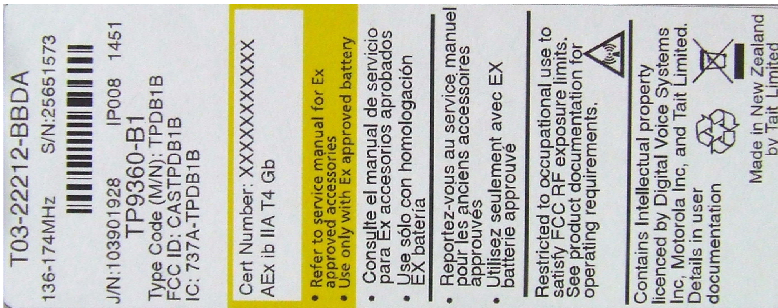
Photograph 02: Compliance Label
