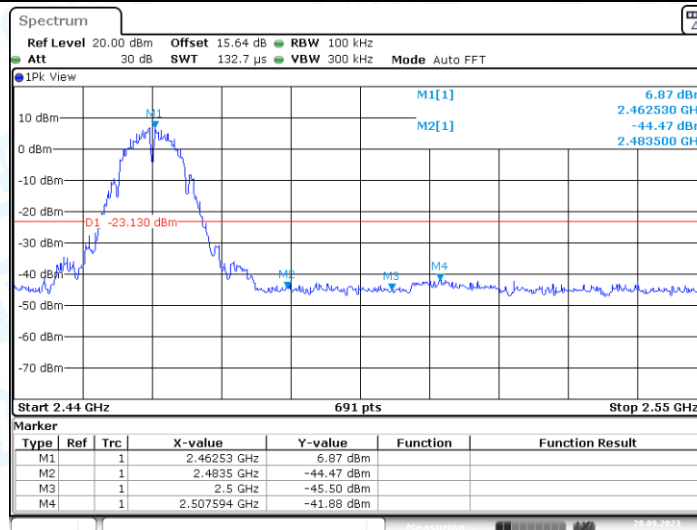
11B_Ant1_High_2462
