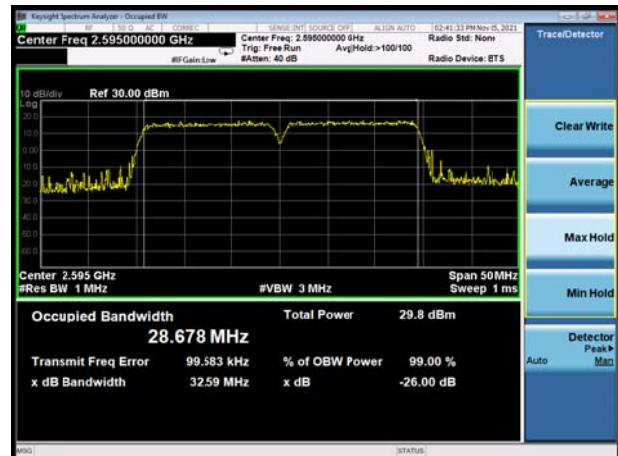
CA_41C 64QAM 15MHz +15MHz
