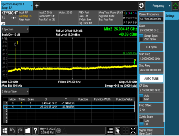
11AX40MIMO-Ant1-2452-242Tone-RU62-1000~26500-PASS
