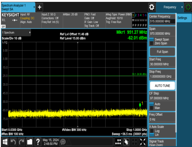
11AX20MIMO-Ant1-2412-106Tone-RU54-30~1000-PASS
