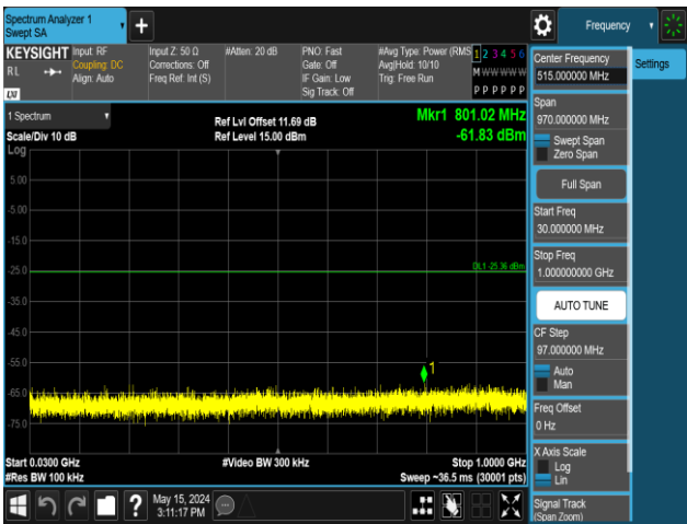
11AX40MIMO-Ant2-2452-242Tone-RU62-30~1000-PASS
