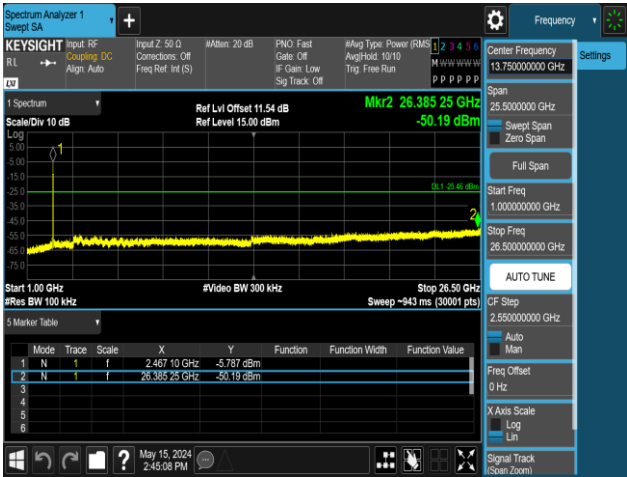
11N40MIMO-Ant1-2452-1000~26500-PASS
