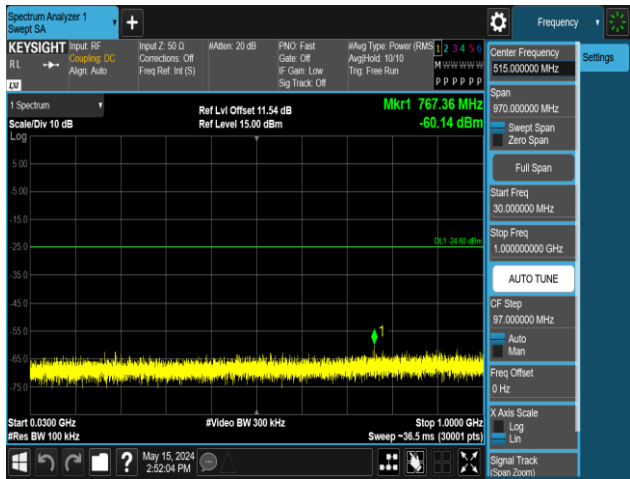
11AX20MIMO-Ant1-2437-106Tone-RU54-30~1000-PASS
