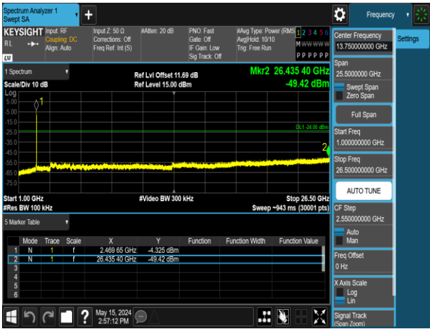
11AX20MIMO-Ant2-2462-106Tone-RU54-1000~26500-PASS
