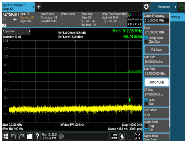
11AX20MIMO-Ant1-2462-106Tone-RU54-30~1000-PASS
