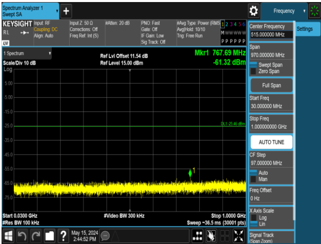
11N40MIMO-Ant1-2452-30~1000-PASS
