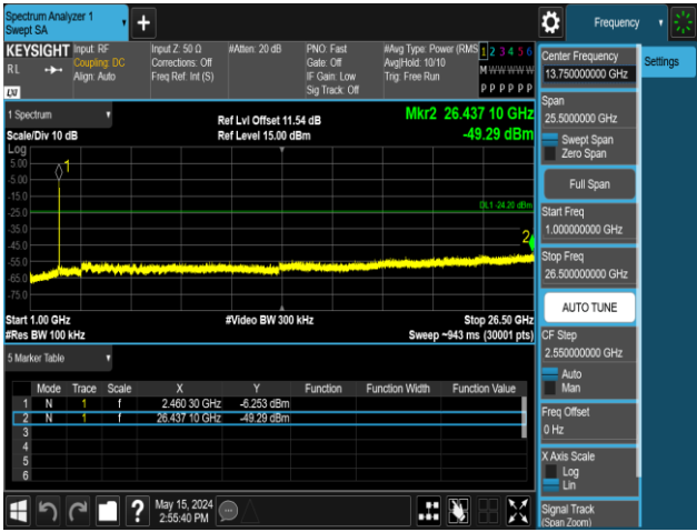
11AX20MIMO-Ant1-2462-106Tone-RU54-1000~26500-PASS
