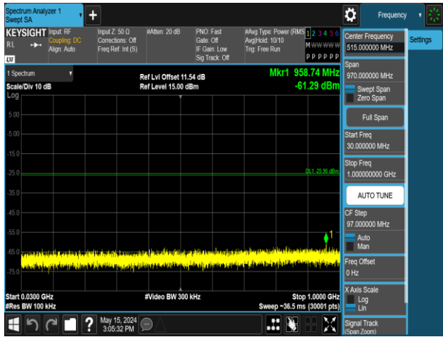
11AX40MIMO-Ant1-2452-242Tone-RU62-30~1000-PASS
