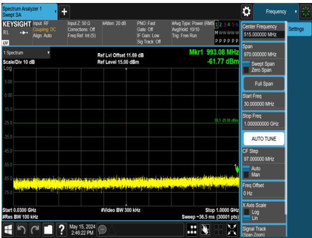
11N40MIMO-Ant2-2452-30~1000-PASS
