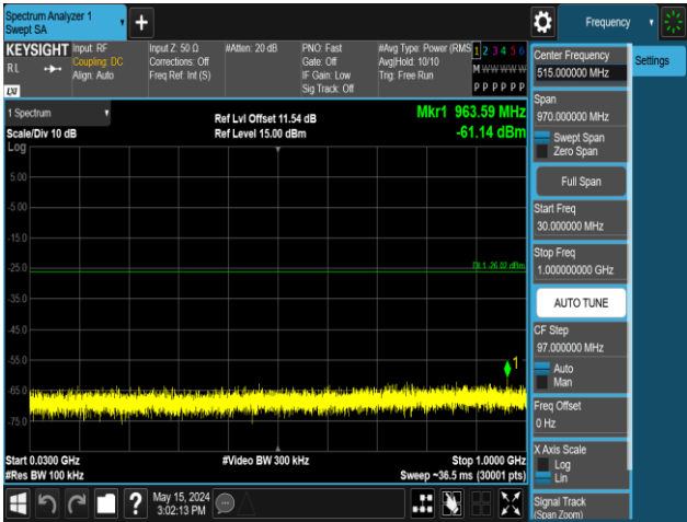
11AX40MIMO-Ant1-2437-242Tone-RU62-30~1000-PASS
