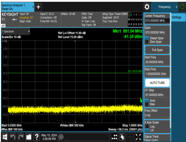
11AX20MIMO-Ant2-2462-106Tone-RU54-30~1000-PASS
