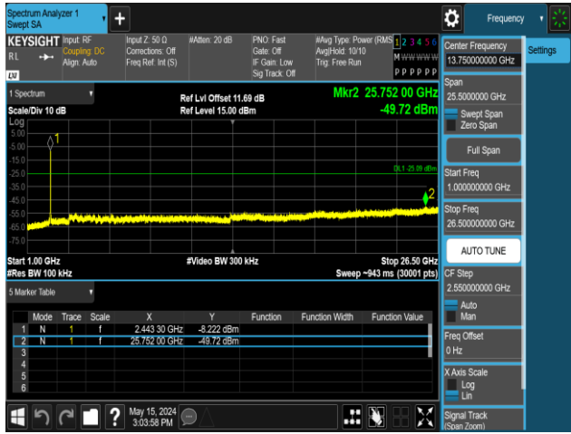
11AX40MIMO-Ant2-2437-242Tone-RU62-1000~26500-PASS
