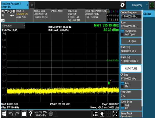
11AX40MIMO-Ant2-2422-242Tone-RU62-30~1000-PASS
