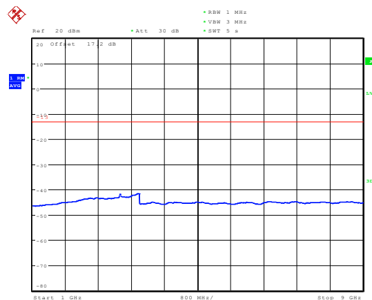
NB-IOT Band 5 CH-Low 1GHz-9GHz
