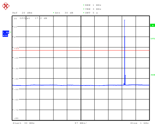
NB-IOT Band 5 CH-Low 30MHz-1GHz
