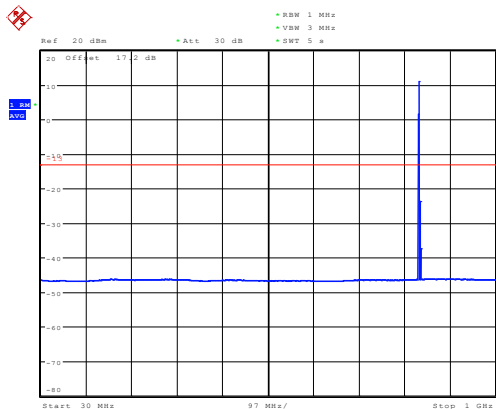
NB-IOT Band 5 CH-Middle 30MHz-1GHz
