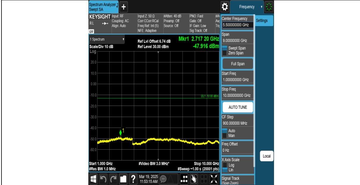
Band26(814-824)-3MHz-16QAM-26775-1RB#14-30-1000-PASS
