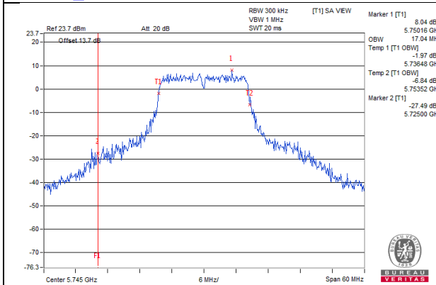
802.11ac(VHT20)_Chain0 / CH149
