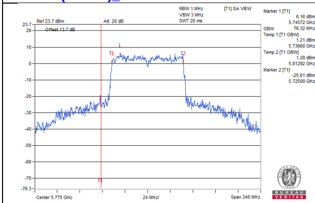
802.11ac(VHT80)_Chain0 / CH155
