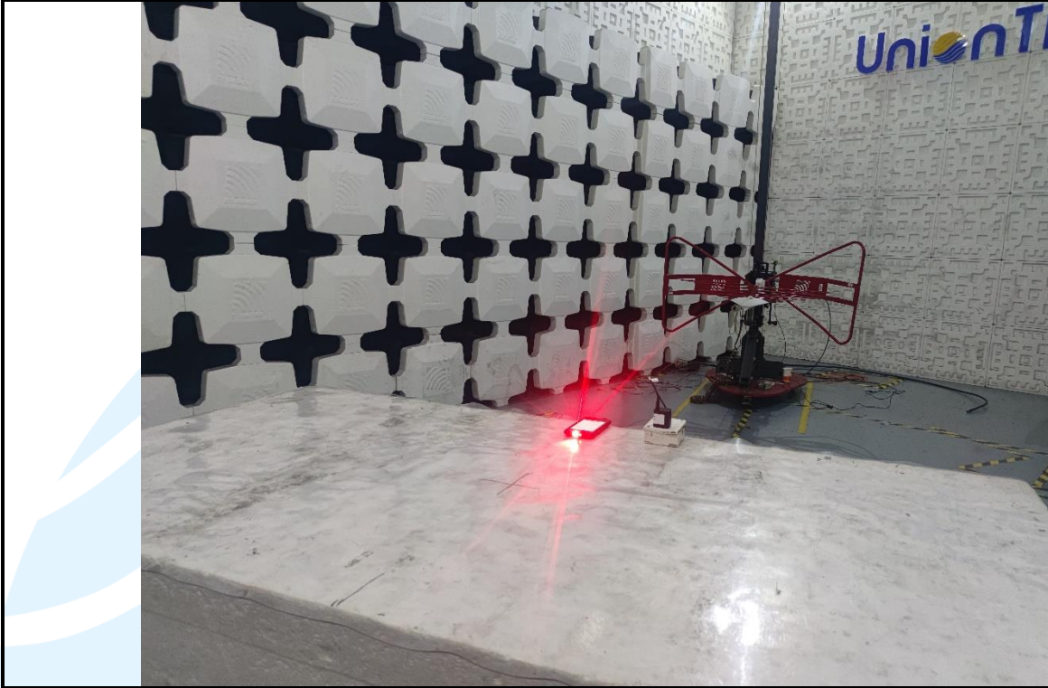
Radiated emission Test Setup-1 (30 MHz~1 GHz) – Test Mode 4
