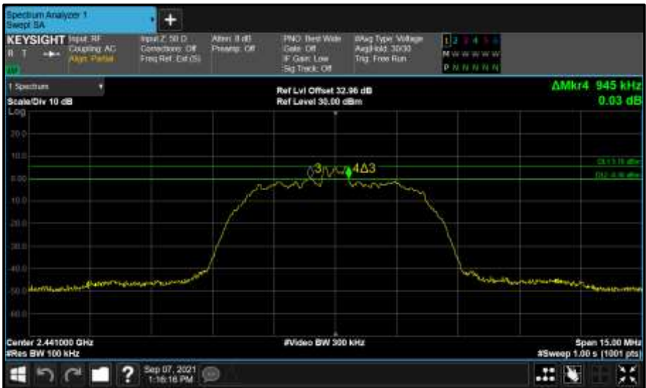
Figure 133 - Core 2 (C) 2441 MHz (CH39) 6 dB Bandwidth
