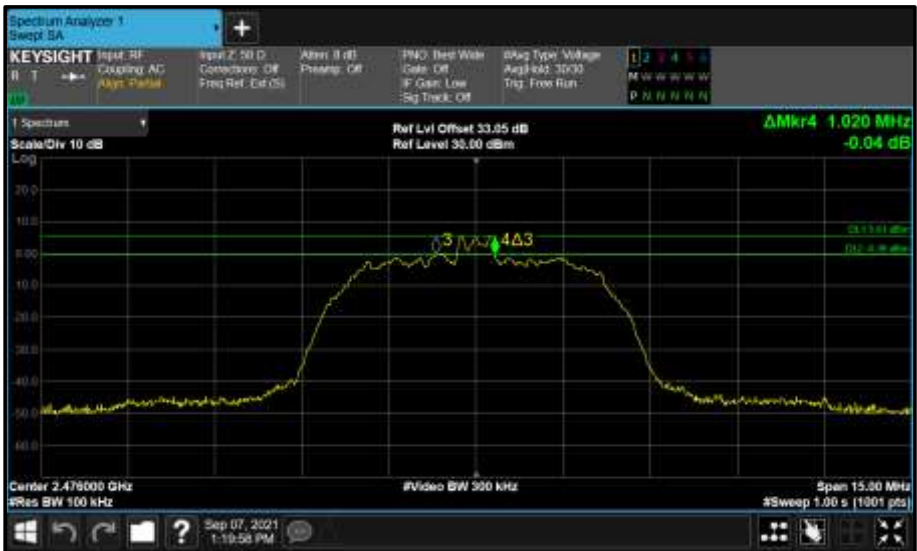
Figure 135 - Core 2 (C) 2476 MHz (CH74) 6 dB Bandwidth
