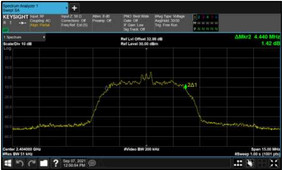
Figure 118 - Core 0 (A) 2404 MHz (CH2) 99% Bandwidth
