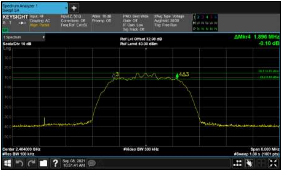
Figure 54 - Core 0 (A) 2404 MHz (CH2) 6 dB Bandwidth
