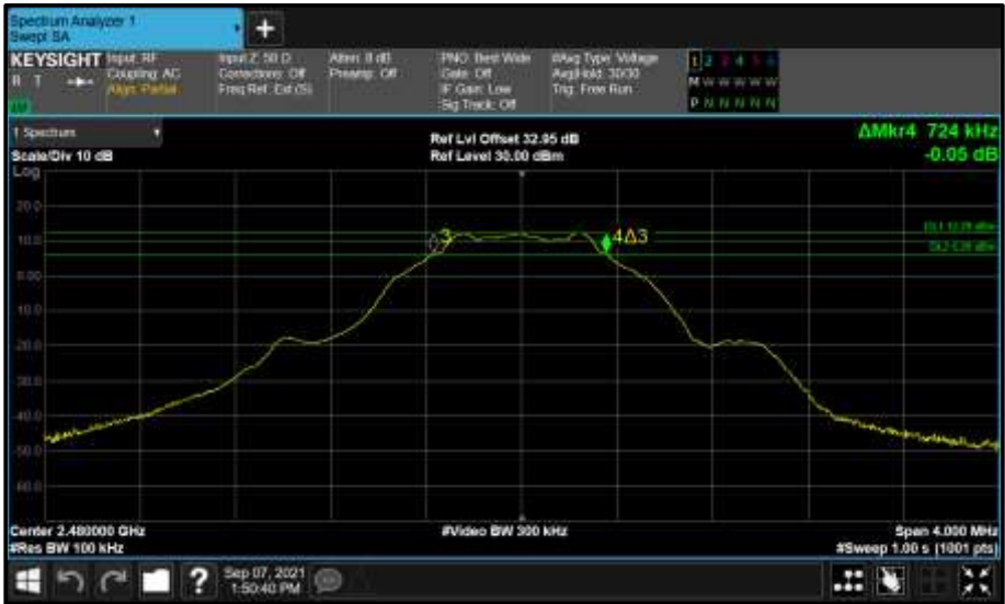
Figure 165 - Core 0 (A) 2480 MHz (CH39) 6 dB Bandwidth
