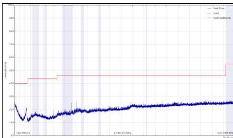
Figure 217 - 2440 MHz (CH17), LE1M, ePA, Core 0 + Core 1, 30 MHz to 1 GHz, Horizontal (Peak)
