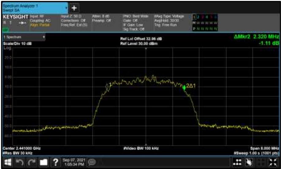
Figure 126 - Core 2 (C) 2441 MHz (CH39) 99% Bandwidth
