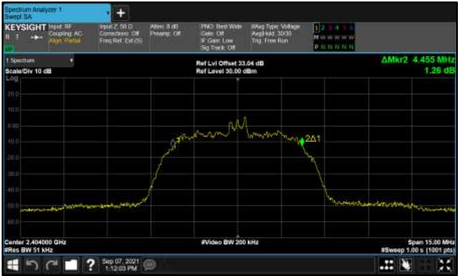
Figure 130 - Core 2 (C) 2404 MHz (CH2) 99% Bandwidth
