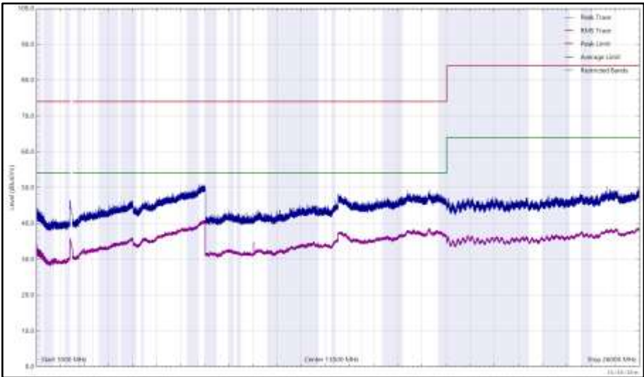
Figure 240 - 2476 MHz (CH74), HDR4, ePA, Core 0 + Core 1, 1 GHz to 26 GHz, Vertical
