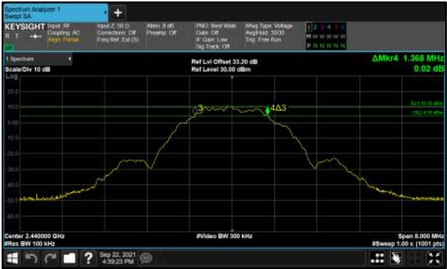
Figure 108 - Core 1 (B) 2440 MHz (CH17) 6 dB Bandwidth
