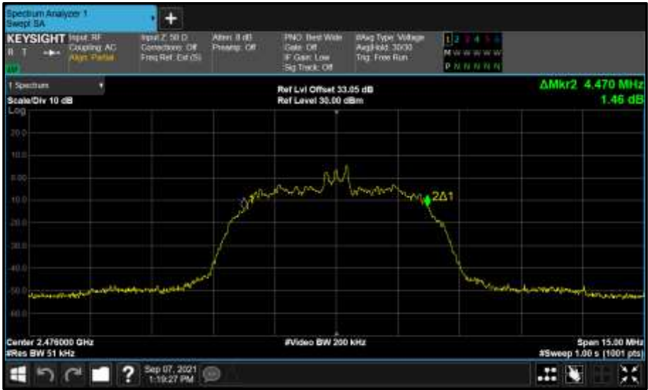
Figure 134 - Core 2 (C) 2476 MHz (CH74) 99% Bandwidth
