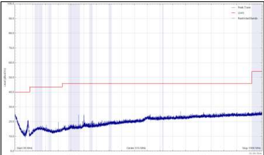
Figure 225 - 2440 MHz (CH17), LE1M, iPA, Core 2, 30 MHz to 1 GHz, Horizontal (Peak)
