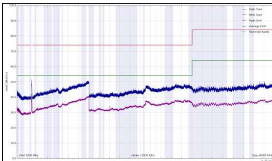
Figure 216 - 2404 MHz (CH2), HDR4, ePA, Core 0 + Core 1, 1 GHz to 26 GHz, Vertical
