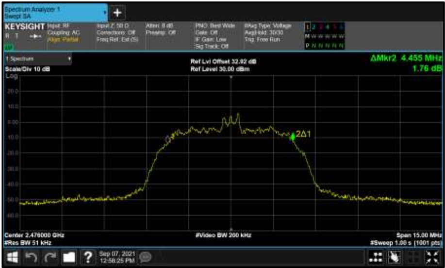
Figure 122 - Core 0 (A) 2476 MHz (CH74) 99% Bandwidth
