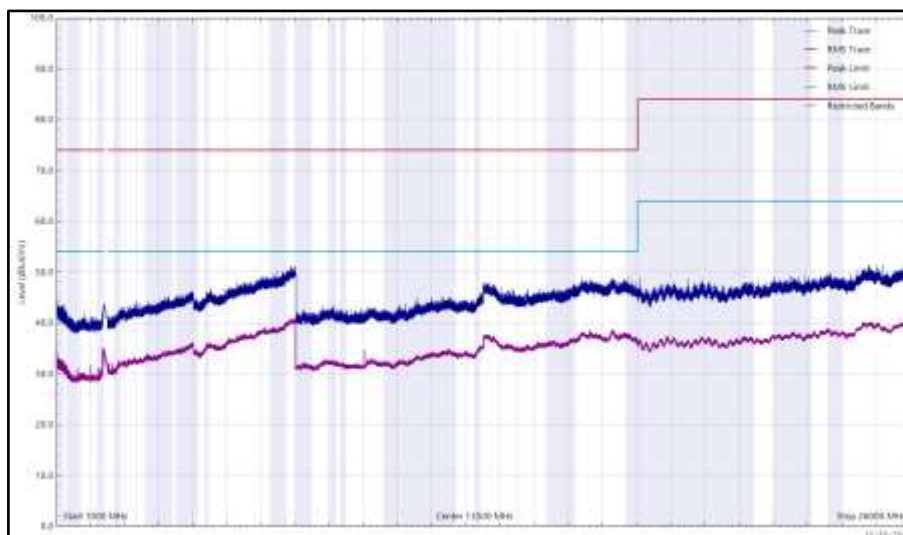
Figure 212 - 2402 MHz (CH37), LE1M, iPA, Core 0 + Core 1, 1 GHz to 26 GHz, Vertical
