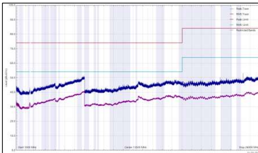
Figure 211 - 2402 MHz (CH37), LE1M, iPA, Core 0 + Core 1, 1 GHz to 26 GHz, Horizontal
