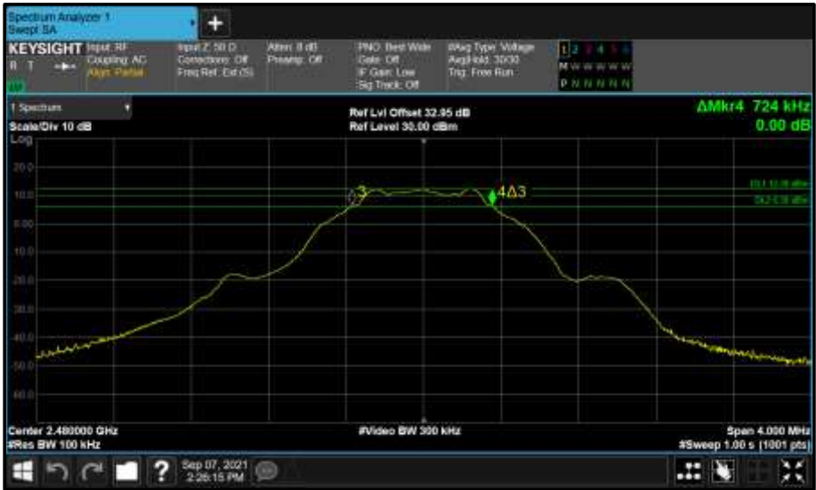
Figure 82 - Core 0 (A) 2480 MHz (CH39) 6 dB Bandwidth
