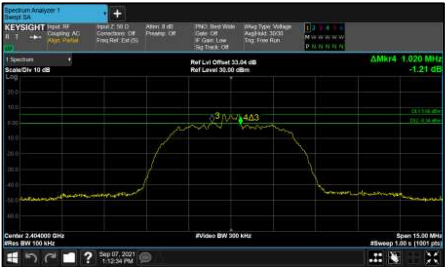
Figure 131 - Core 2 (C) 2404 MHz (CH2) 6 dB Bandwidth
