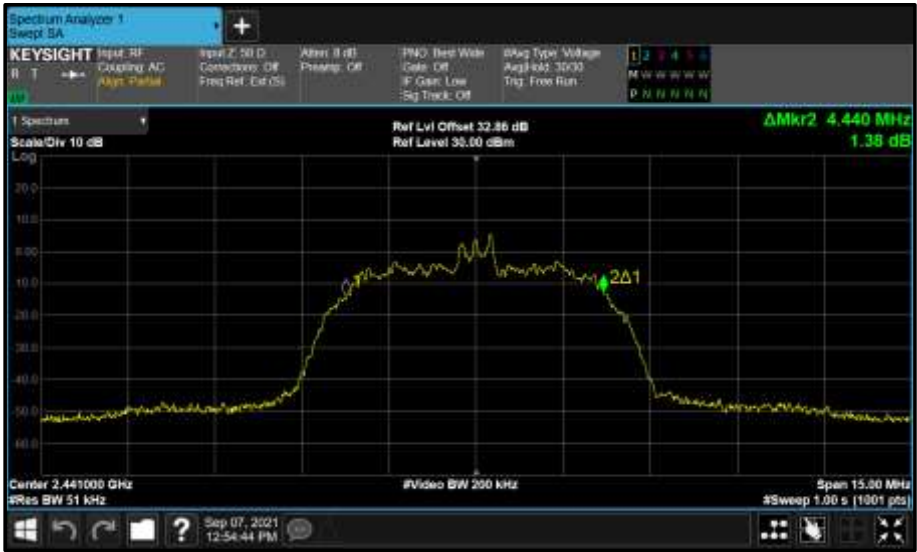
Figure 120 - Core 0 (A) 2441 MHz (CH39) 99% Bandwidth
