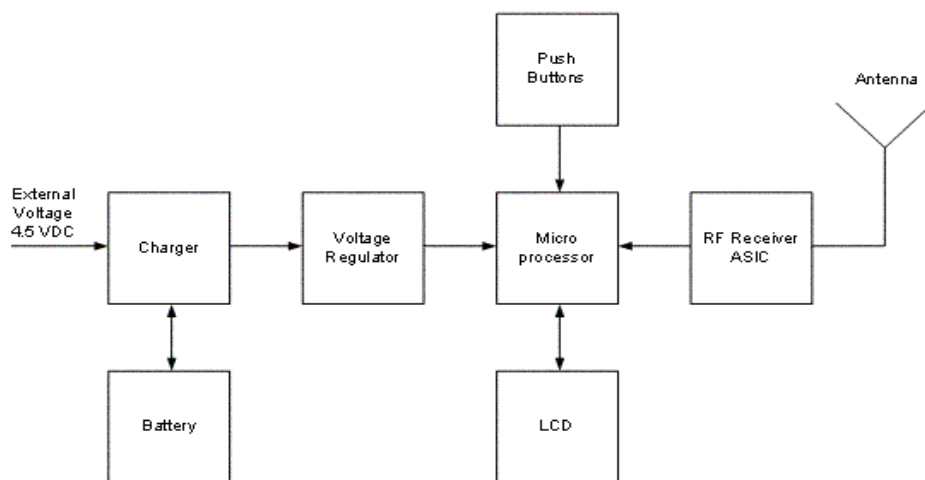
LPU - 800 Block Diagram
