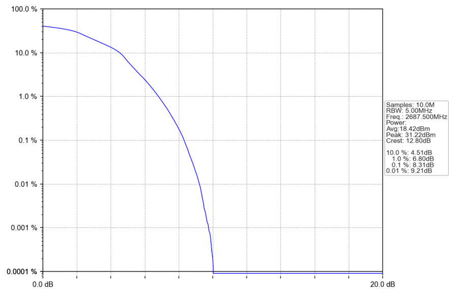
Band41_5MHz_16QAM_HCH_2687.500MHz_RB_25_0_NTNV
