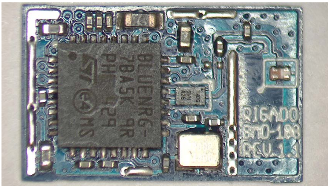
PCB side 1
