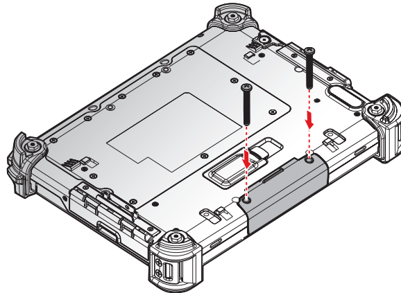
Figure 39. Securing the Screws
