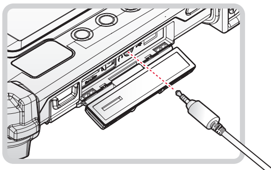
Figure 46. Connect Audio Cabling
