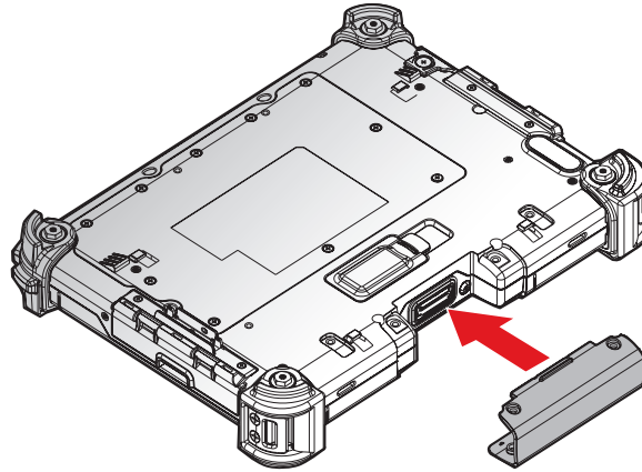
Figure 38. Installing the Snap-on Module Connector Cover
