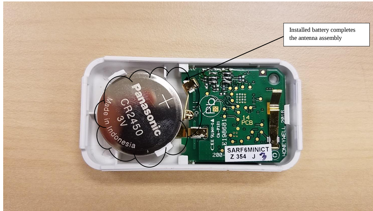
PCB Installed in Enclosure with Battery
