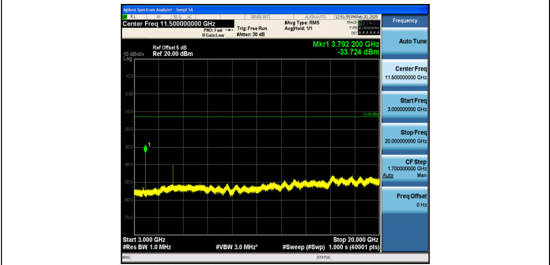
Band25_20MHz_16QAM_26590_1RB#0_3000~20000_3000~20000
