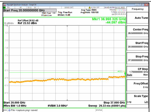
48C-20G-37G / 5+20MHz / QPSK / High CH / 1#24-1#0
