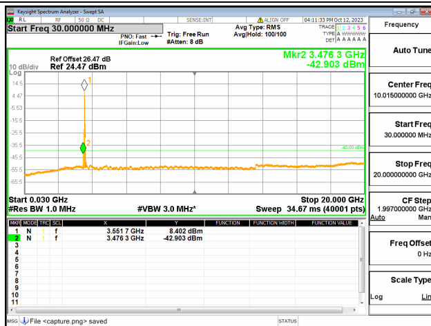
48C-30M-20G / 20+20MHz / QPSK / Low CH / 1#0-1#99
