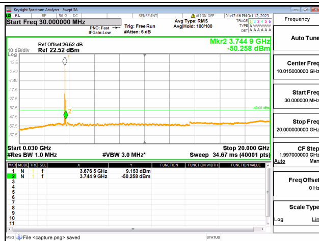
48C-30M-20G / 20+5MHz / QPSK / High CH / 1#0-1#24
