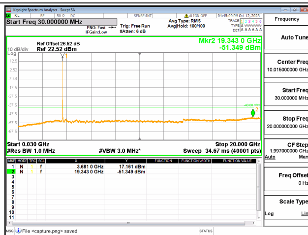
48C-30M-20G / 5+20MHz / QPSK / High CH / 1#24-1#0
