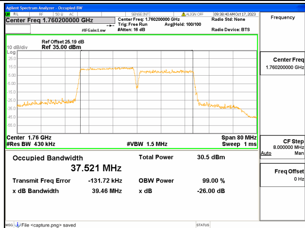
66C / 20+20MHz / 64QAM/ High CH
