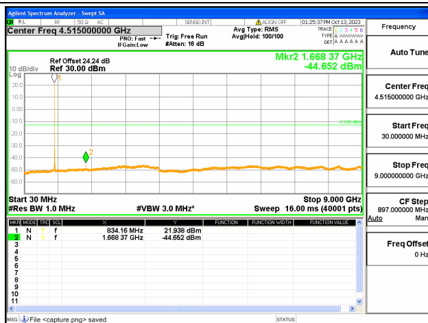
5B / 5+10MHz / QPSK / Mid CH / 1#24-1#0
