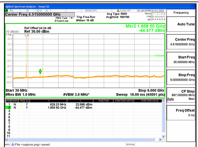
5B / 5+10MHz / QPSK / Low CH / 1#24-1#0
