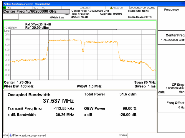
66C / 20+20MHz / QPSK/ High CH
