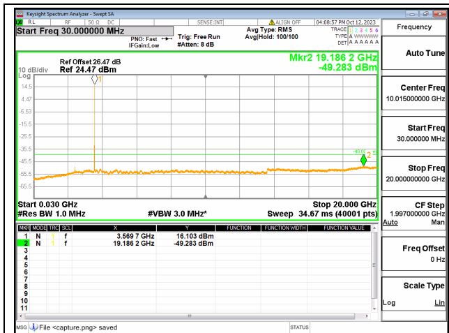
48C-30M-20G / 20+15MHz / QPSK / Low CH / 1#99-1#0
