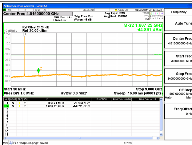
5B / 10+5MHz / QPSK / Low CH / 1#49-1#0
