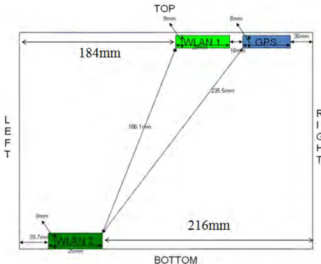
Fig.14 Antenna position of EUT (Front view)
