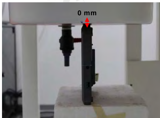
Fig.9 EUT Bottom side with optional battery to flat phantom
