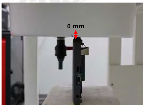
Fig.5 EUT Top side with optional battery to flat phantom
