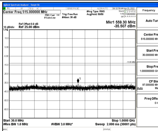
Band25-15MHz-QPSK-26365-1-0-Low-30-1000--35.51-PASS
