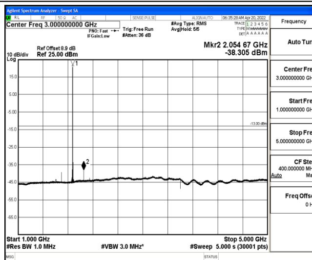
Band25-15MHz-16QAM-26365-1-0-Low-1000-5000--38.31-PASS
