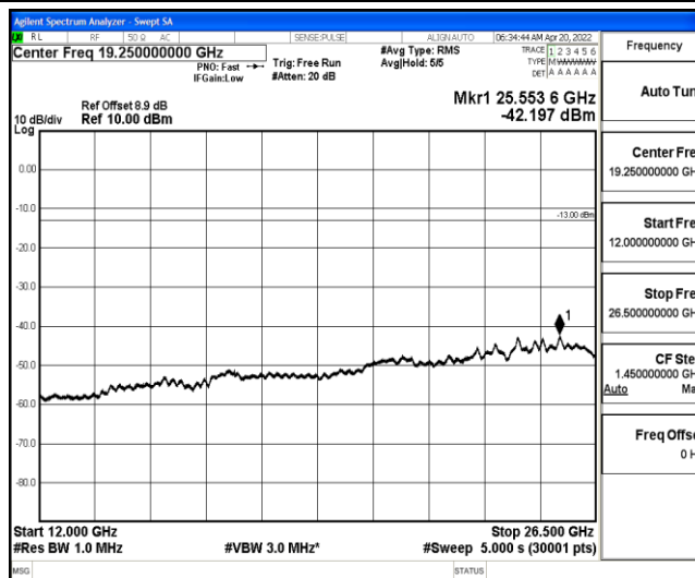
Band25-15MHz-QPSK-26365-1-0-Low-12000-26500--42.2-PASS
