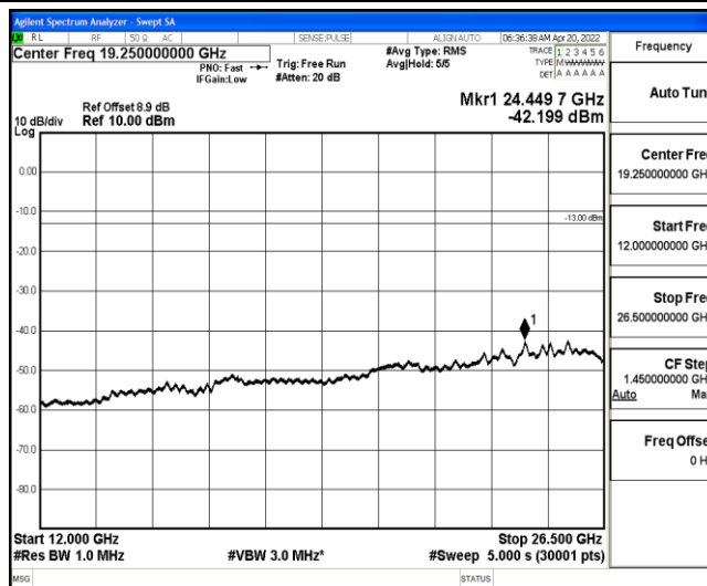
Band25-15MHz-16QAM-26365-1-0-Low-12000-26500--42.2-PASS
