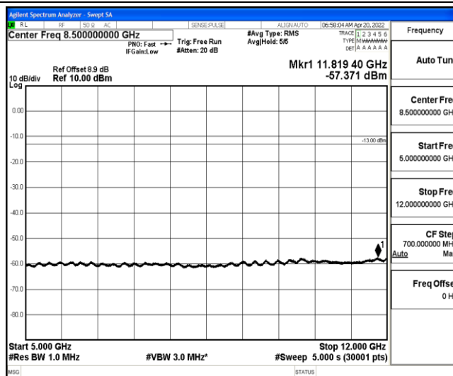
Band25-20MHz-16QAM-26365-1-0-Low-5000-12000--57.37-PASS
