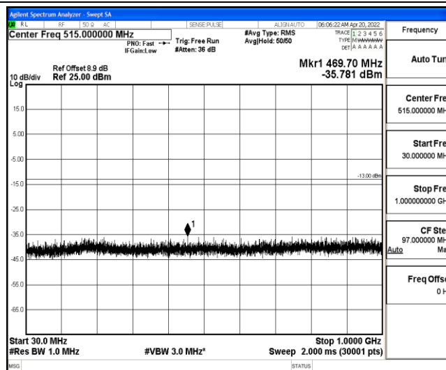
Band25-10MHz-16QAM-26090-1-0-Low-30-1000--35.78-PASS
