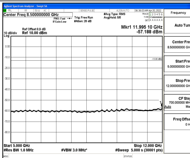
Band25-15MHz-16QAM-26365-1-0-Low-5000-12000--57.19-PASS
