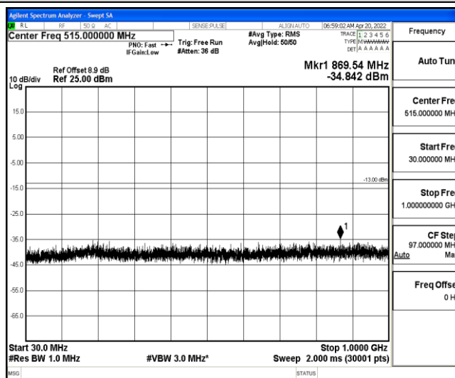
Band25-20MHz-QPSK-26590-1-0-High-30-1000--34.84-PASS
