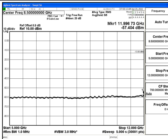
Band25-20MHz-QPSK-26590-1-0-High-5000-12000--57.4-PASS
