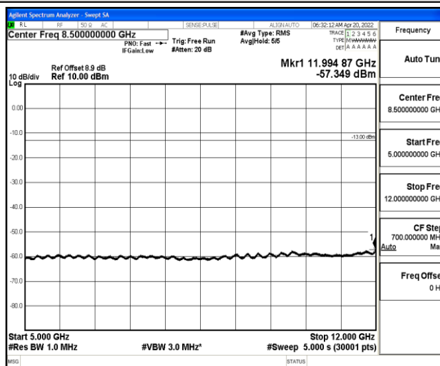
Band25-15MHz-16QAM-26115-1-0-Low-5000-12000--57.35-PASS
