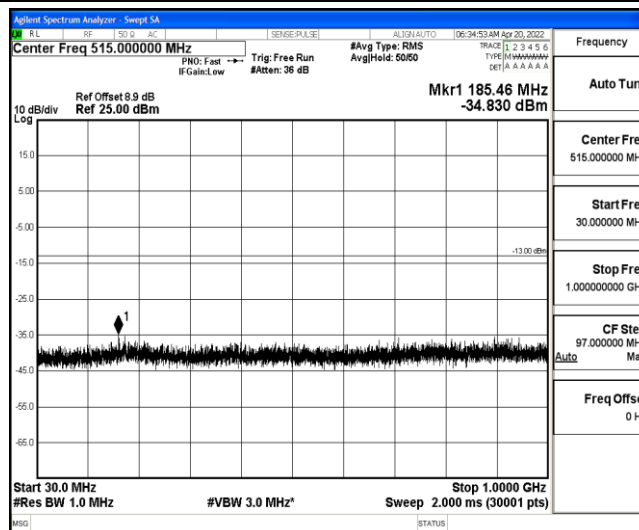
Band25-15MHz-16QAM-26365-1-0-Low-30-1000--34.83-PASS
