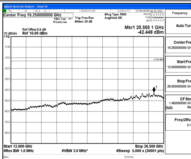
Band25-20MHz-QPSK-26590-1-0-High-12000-26500--42.45-PASS
