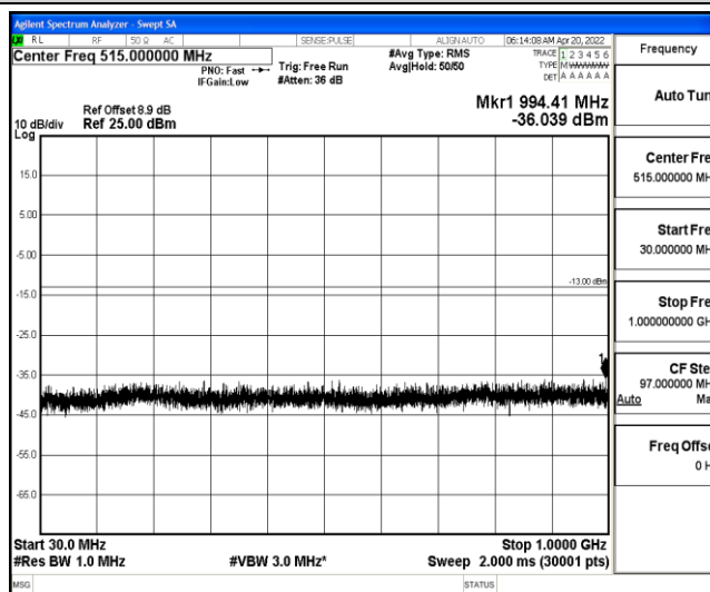
Band25-10MHz-16QAM-26640-1-0-High-30-1000--36.04-PASS
