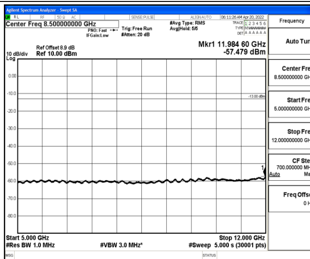
Band25-10MHz-16QAM-26365-1-0-Low-5000-12000--57.48-PASS
