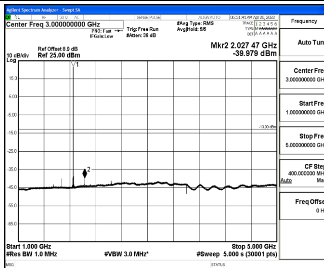
Band25-20MHz-QPSK-26140-1-0-Low-1000-5000--39.98-PASS
