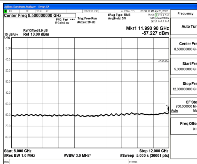
Band25-15MHz-QPSK-26115-1-0-Low-5000-12000--57.23-PASS
