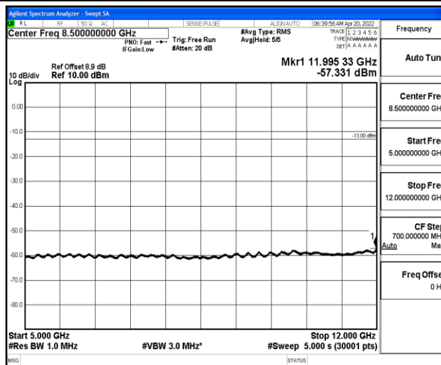
Band25-15MHz-16QAM-26615-1-0-High-5000-12000--57.33-PASS
