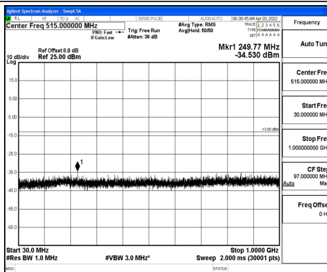
Band25-15MHz-16QAM-26615-1-0-High-30-1000--34.53-PASS
