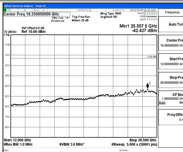
Band25-20MHz-QPSK-26140-1-0-Low-12000-26500--42.43-PASS
