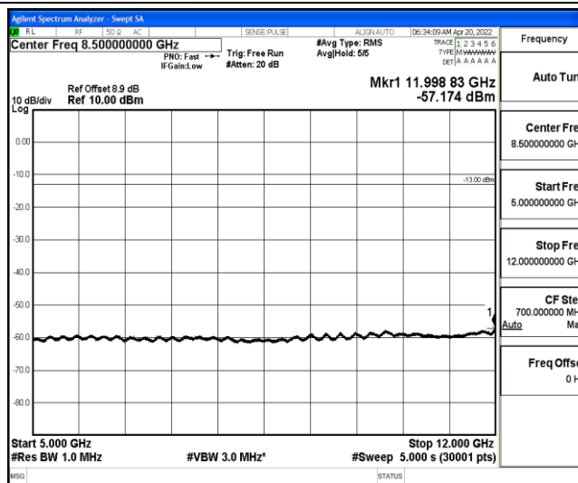
Band25-15MHz-QPSK-26365-1-0-Low-5000-12000--57.17-PASS
