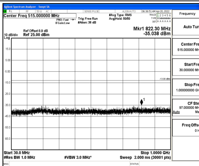
Band25-15MHz-QPSK-26615-1-0-High-30-1000--35.04-PASS
