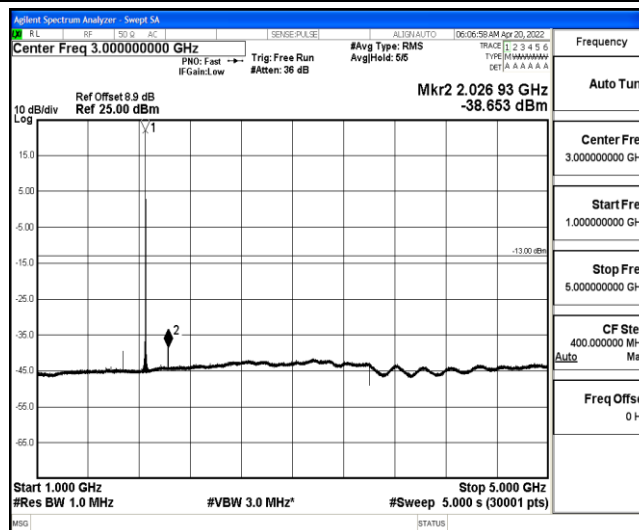
Band25-10MHz-16QAM-26090-1-0-Low-1000-5000--38.65-PASS
