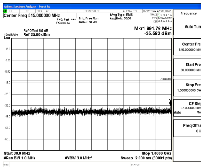
Band25-15MHz-16QAM-26115-1-0-Low-30-1000--35.58-PASS
