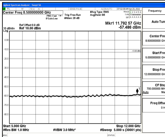
Band25-20MHz-16QAM-26590-1-0-High-5000-12000--57.49-PASS
