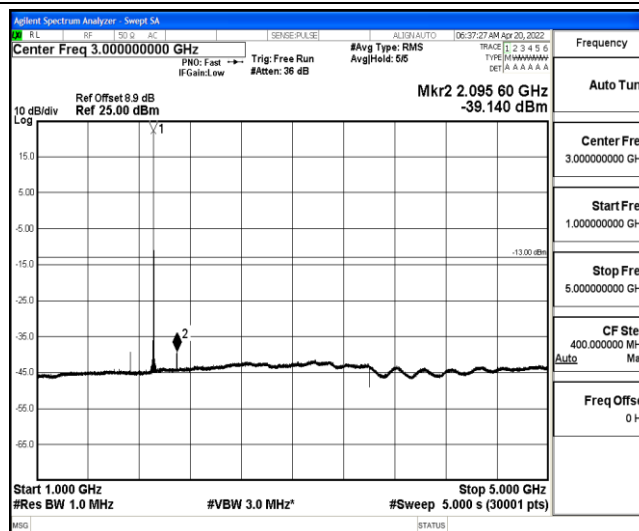
Band25-15MHz-QPSK-26615-1-0-High-1000-5000--39.14-PASS
