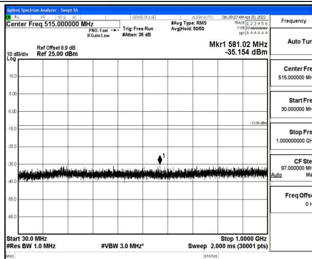
Band25-15MHz-QPSK-26115-1-0-Low-30-1000--35.15-PASS
