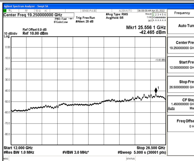
Band25-10MHz-16QAM-26090-1-0-Low-12000-26500--42.47-PASS
