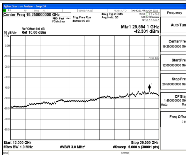
Band25-15MHz-16QAM-26615-1-0-High-12000-26500--42.3-PASS
