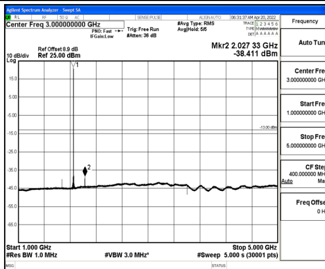
Band25-15MHz-16QAM-26115-1-0-Low-1000-5000--38.41-PASS
