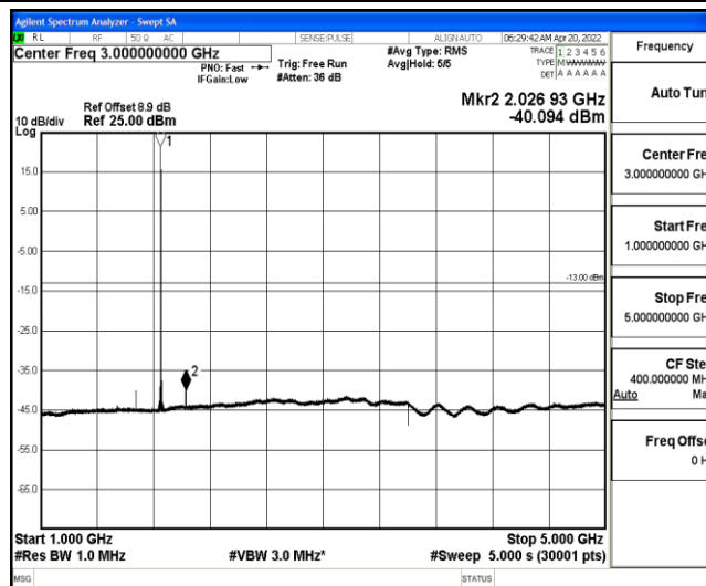
Band25-15MHz-QPSK-26115-1-0-Low-1000-5000--40.09-PASS
