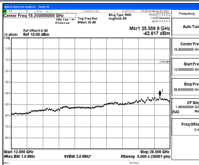
Band25-20MHz-16QAM-26590-1-0-High-12000-26500--42.62-PASS
