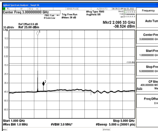
Band25-15MHz-16QAM-26615-1-0-High-1000-5000--38.52-PASS
