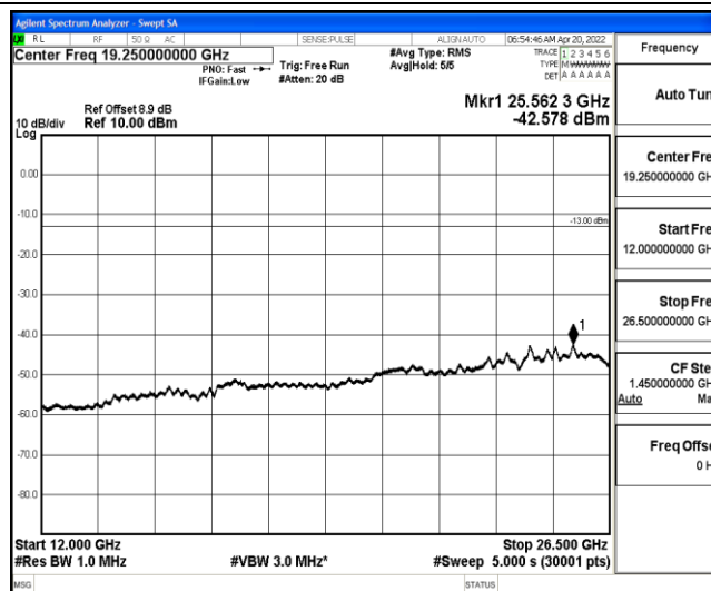
Band25-20MHz-16QAM-26140-1-0-Low-12000-26500--42.58-PASS
