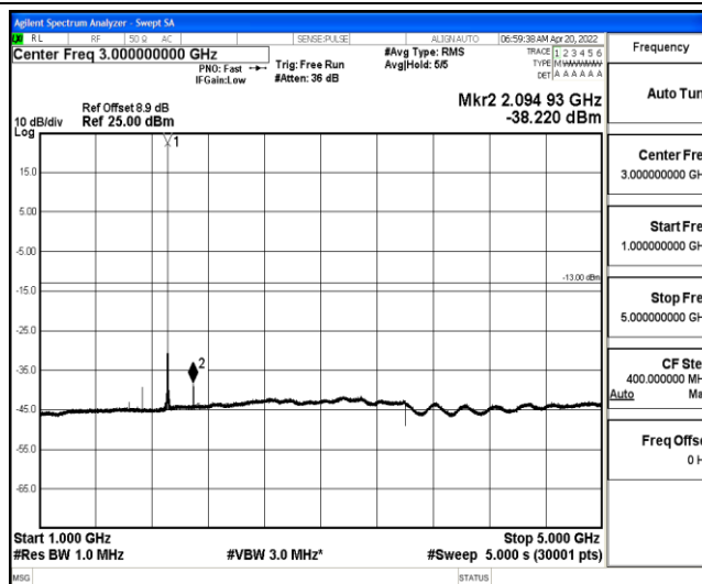
Band25-20MHz-QPSK-26590-1-0-High-1000-5000--38.22-PASS
