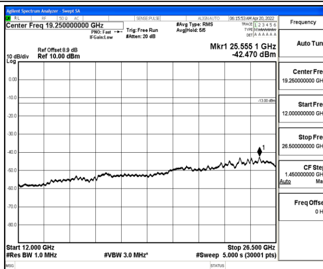
Band25-10MHz-16QAM-26640-1-0-High-12000-26500--42.47-PASS
