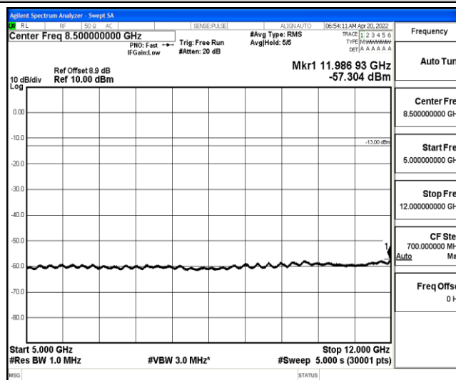
Band25-20MHz-16QAM-26140-1-0-Low-5000-12000--57.3-PASS
