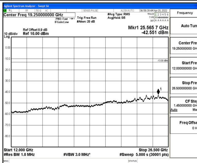
Band25-20MHz-16QAM-26365-1-0-Low-12000-26500--42.55-PASS
