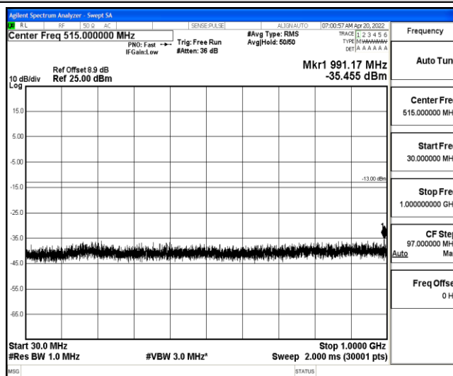
Band25-20MHz-16QAM-26590-1-0-High-30-1000--35.46-PASS
