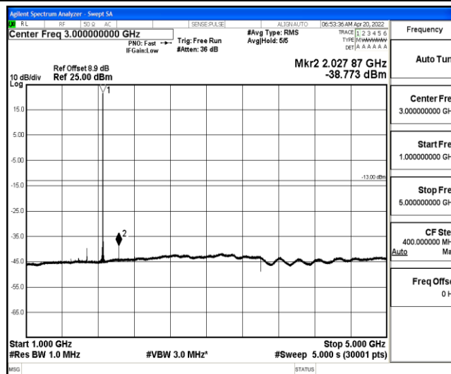
Band25-20MHz-16QAM-26140-1-0-Low-1000-5000--38.77-PASS
