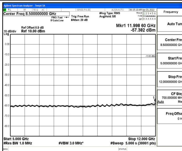
Band25-10MHz-16QAM-26640-1-0-High-5000-12000--57.38-PASS
