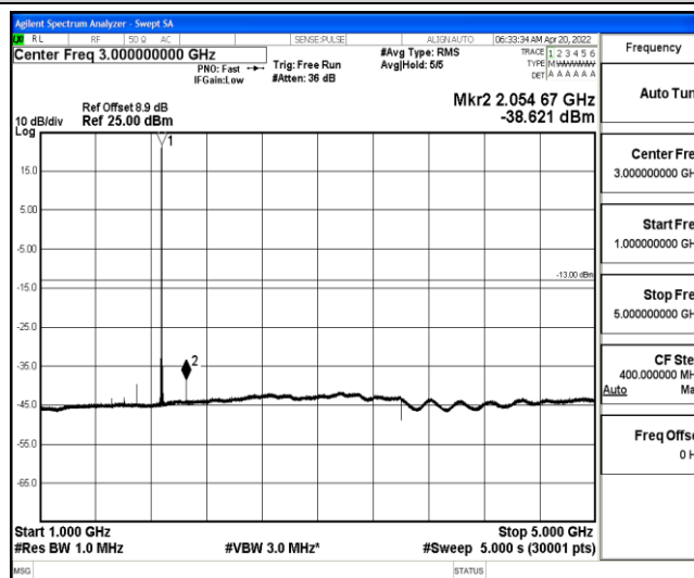
Band25-15MHz-QPSK-26365-1-0-Low-1000-5000--38.62-PASS
