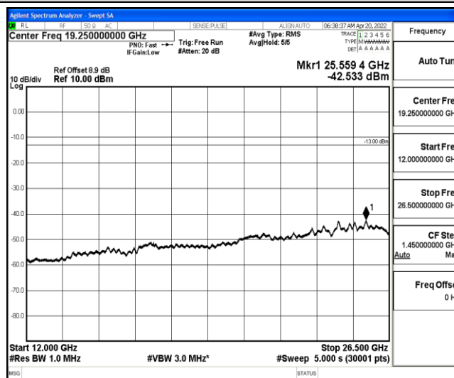
Band25-15MHz-QPSK-26615-1-0-High-12000-26500--42.53-PASS
