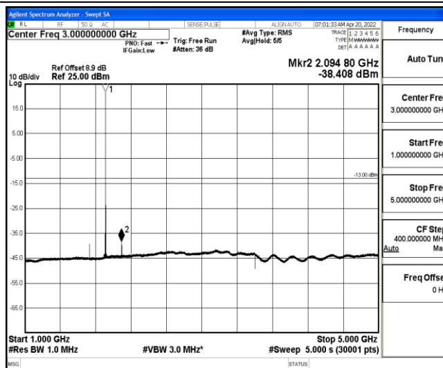
Band25-20MHz-16QAM-26590-1-0-High-1000-5000--38.41-PASS
