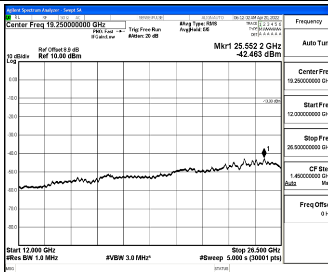
Band25-10MHz-16QAM-26365-1-0-Low-12000-26500--42.46-PASS
