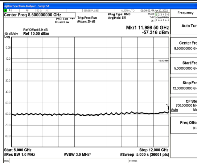
Band25-15MHz-QPSK-26615-1-0-High-5000-12000--57.32-PASS
