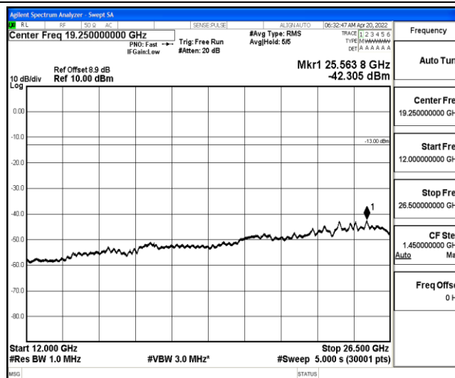
Band25-15MHz-16QAM-26115-1-0-Low-12000-26500--42.31-PASS
