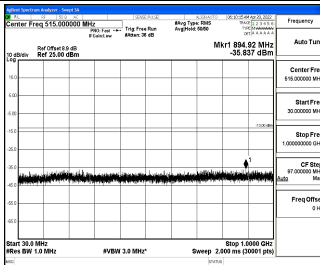
Band25-10MHz-16QAM-26365-1-0-Low-30-1000--35.84-PASS
