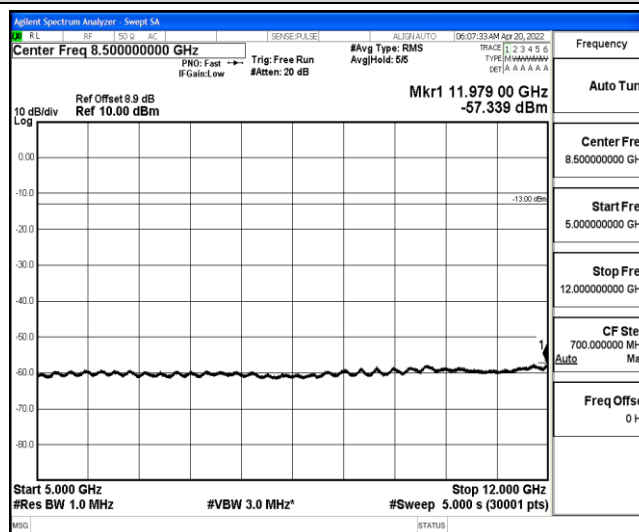
Band25-10MHz-16QAM-26090-1-0-Low-5000-12000--57.34-PASS
