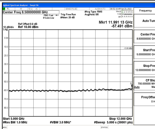
Band25-20MHz-QPSK-26140-1-0-Low-5000-12000--57.49-PASS
