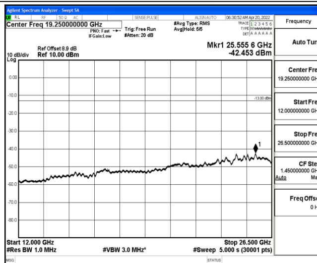
Band25-15MHz-QPSK-26115-1-0-Low-12000-26500--42.45-PASS
