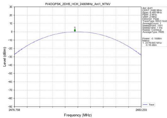
Pi/4DQPSK_2DH5_HCH_2480MHz_Ant1_NTNV
