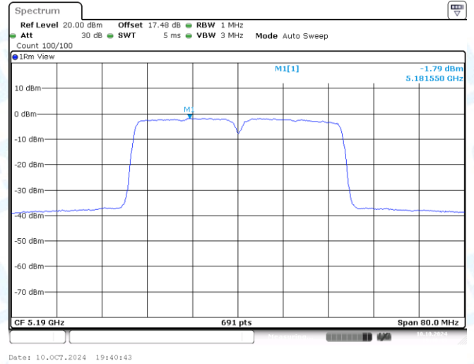
11AC40MIMO-Ant2-5190-PASS
