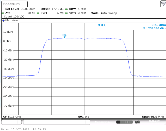
11AX20MIMO-Ant1-5180-PASS
