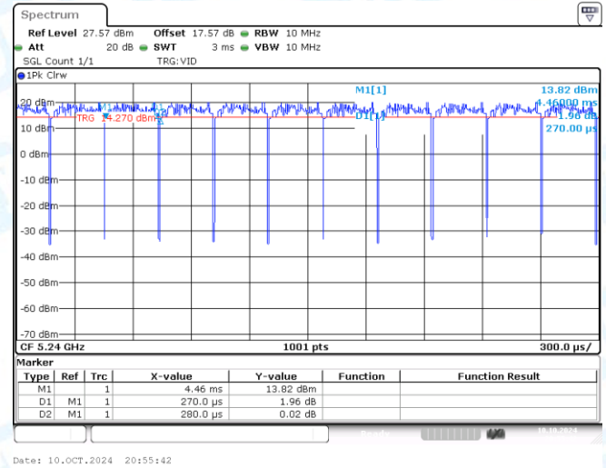
NTNV-11AX20MIMO-Ant2-5240
