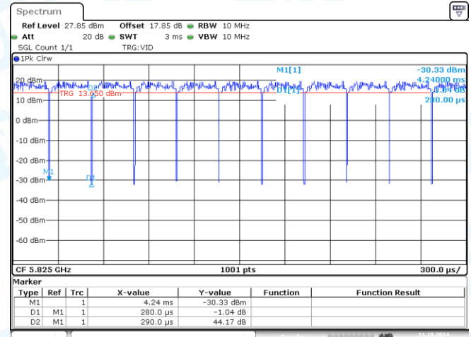
NTVN-11AX20MIMO-Ant2-5825
