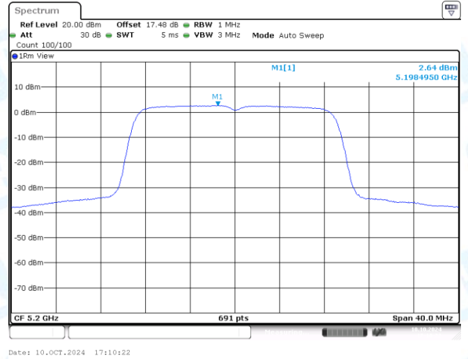
11N20MIMO-Ant2-5200-PASS
