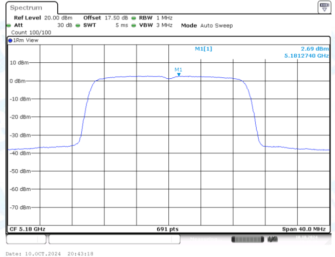
11AX20MIMO-Ant2-5180-PASS
