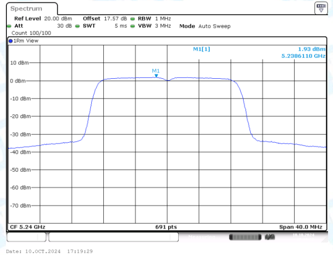
11N20MIMO-Ant2-5240-PASS
