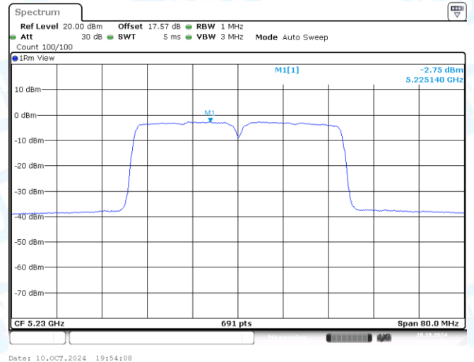
11AC40MIMO-Ant2-5230-PASS
