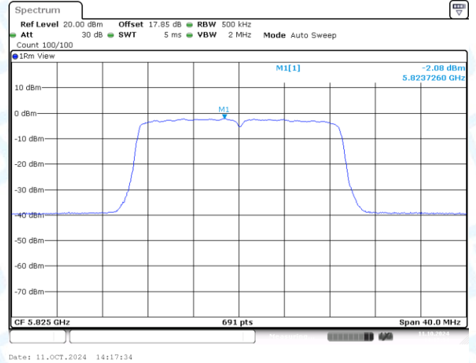
11AC20MIMO-Ant2-5825-PASS
