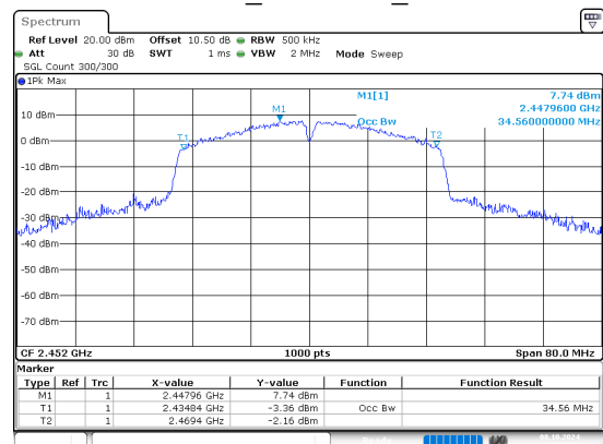
802.11n40_2452MHz_Chain 0
