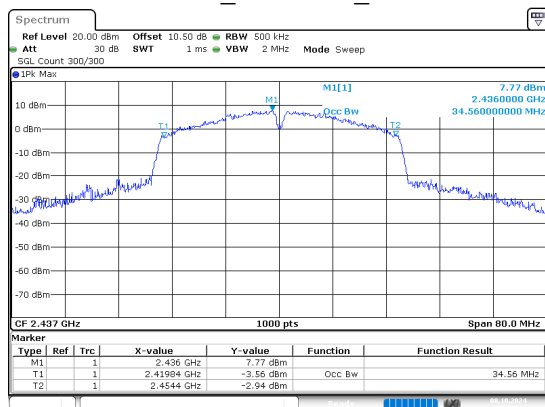
802.11n40_2437MHz_Chain 0
