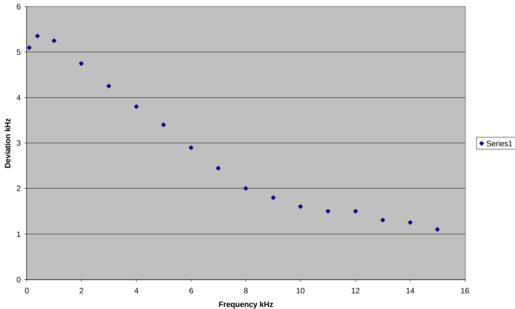
LT800 Frequency Response Ch. 1K
