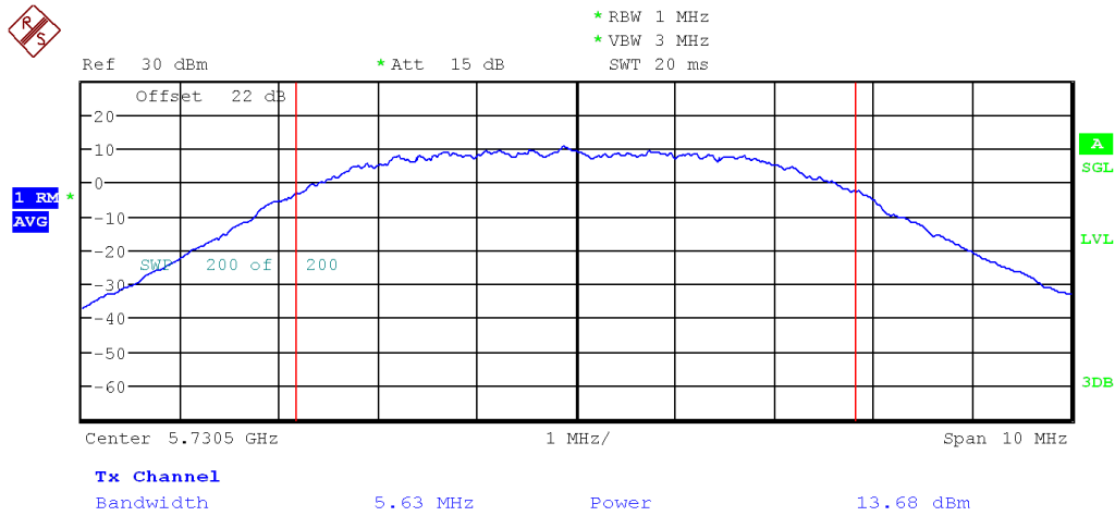
Figure 5: FCC Uncorrelated Max Conducted Power-5730.5 MHz-802.11n-MCS 0-5MHz-Ch0
