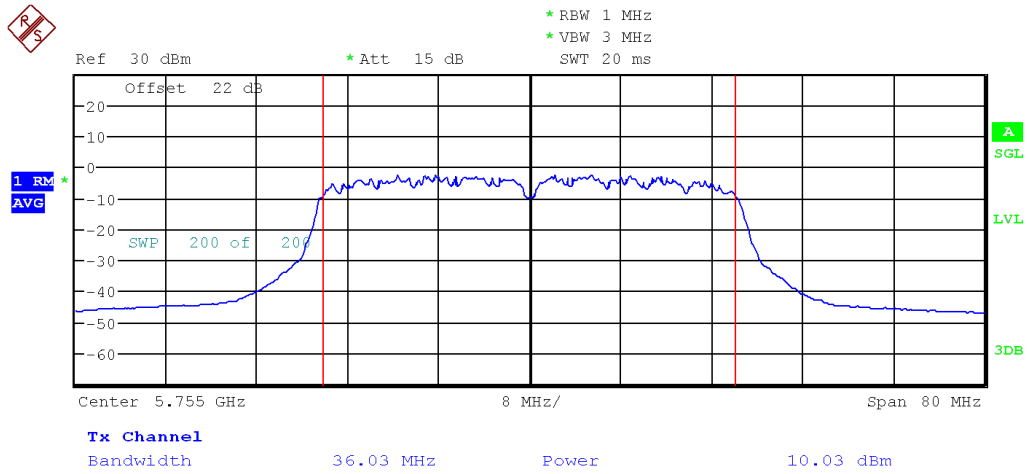
Figure 9: FCC Uncorrelated Max Conducted Power-5755 MHz-802.11ac-MCS 0-40MHz-Ch0
