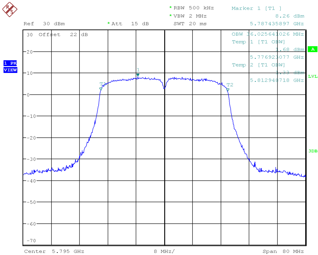
Figure 20: Occupied Bandwidth-5795 MHz-802.11n HT40
