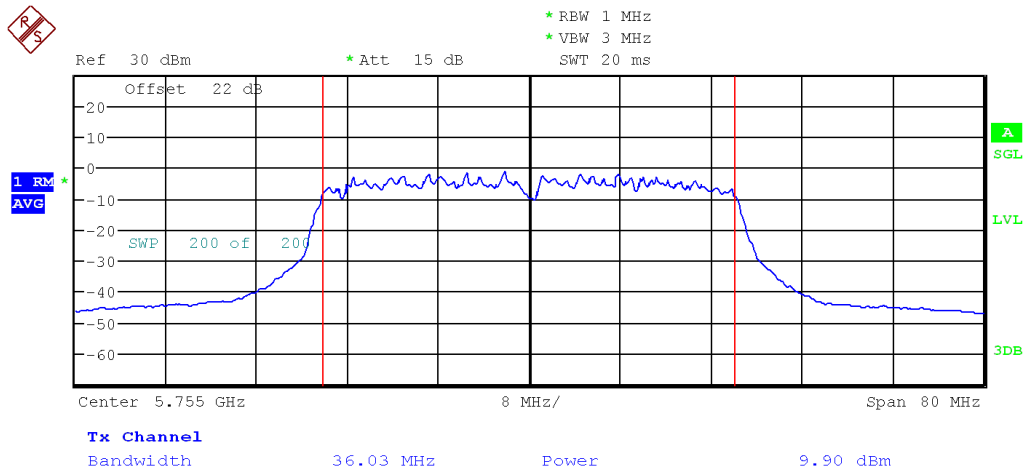
Figure 10: FCC Uncorrelated Max Conducted Power-5755 MHz-802.11ac-MCS 0-40MHz-Ch1
