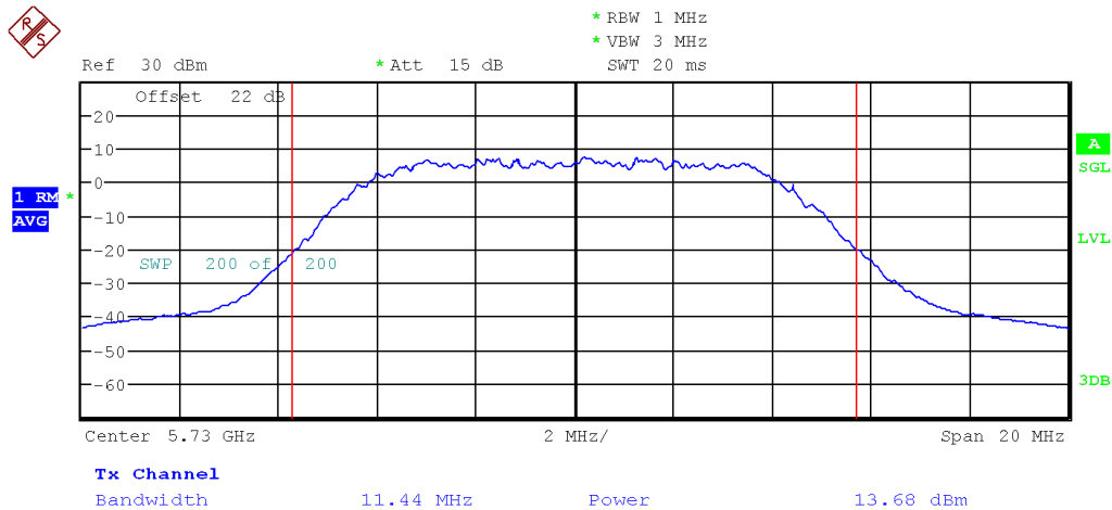
Figure 8: FCC Uncorrelated Max Conducted Power-5730 MHz-802.11a-6 Mbps -10MHz-Ch1
