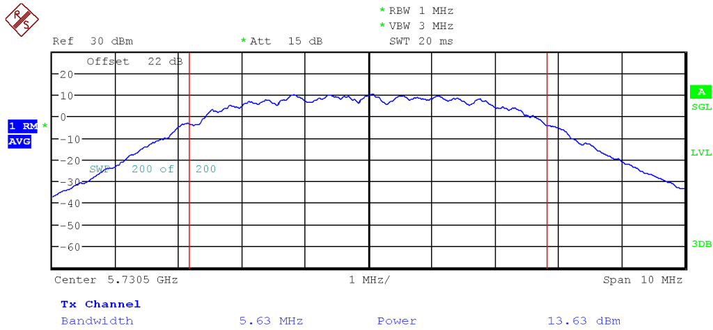
Figure 6: FCC Uncorrelated Max Conducted Power-5730.5 MHz-802.11n-MCS 0-5MHz-Ch1
