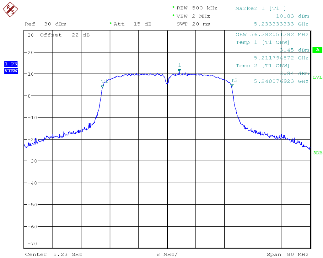
Figure 19: Occupied Bandwidth-5230 MHz-802.11n HT40
