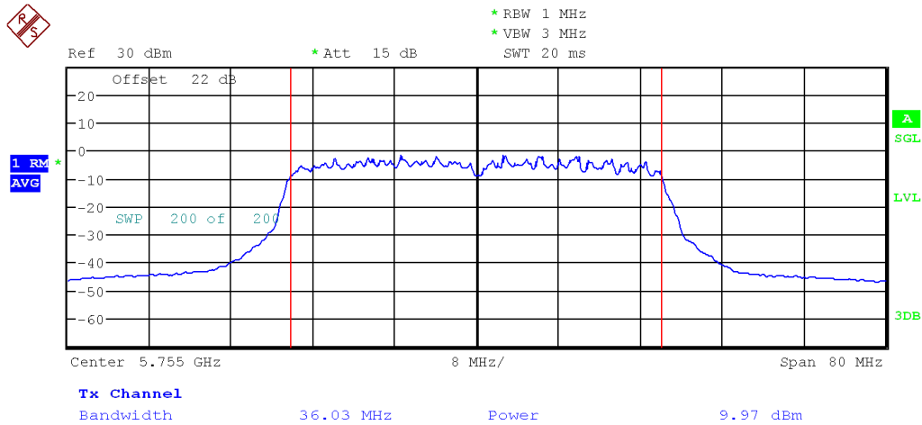
Figure 14: FCC Uncorrelated Max Conducted Power-5755 MHz-802.11ac VHT-MCS 0-40MHz- Ch1
