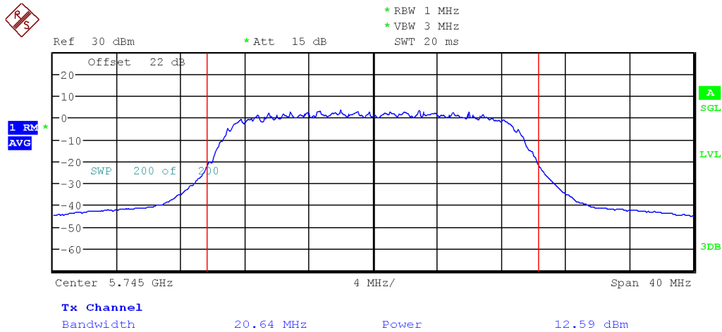
Figure 12: FCC Uncorrelated Max Conducted Power-5745 MHz-802.11ac VHT-MCS 0-20MHz- Ch1
