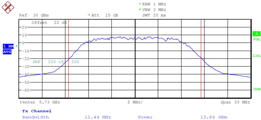
Figure 7: FCC Uncorrelated Max Conducted Power-5730 MHz-802.11a-6 Mbps -10MHz-Ch0
