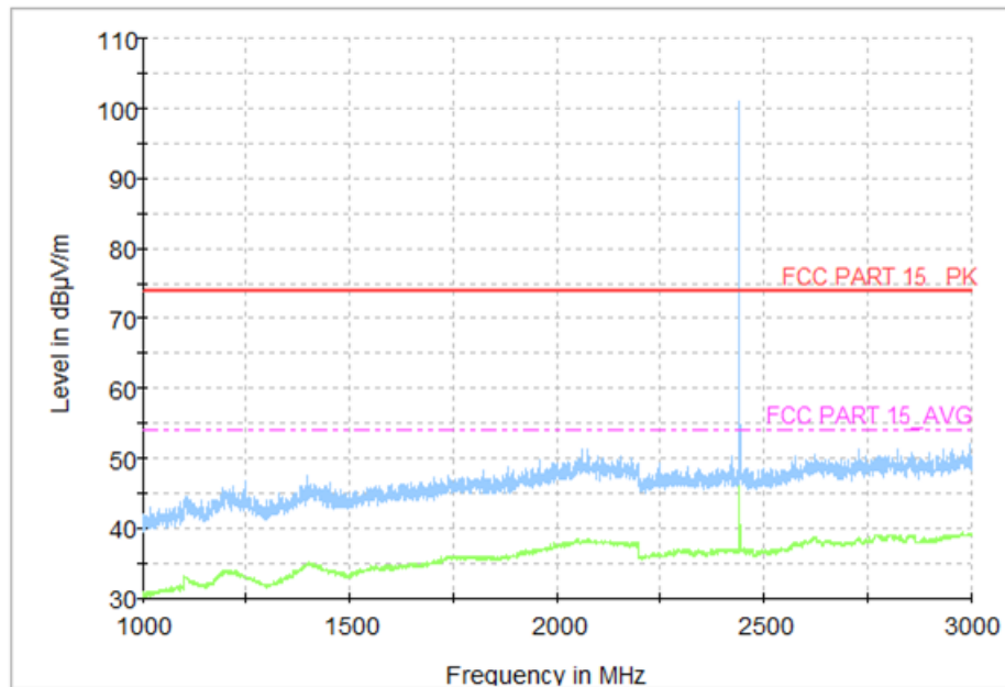
Fig. 53 Radiated Spurious Emission (GFSK, Ch39, 1 GHz ~3 GHz)
