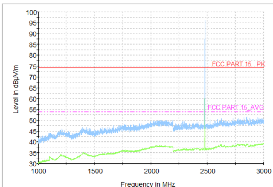
Fig. 63 Radiated Spurious Emission ( \pi/4 DQPSK, Ch78, 1 GHz ~3 GHz)
