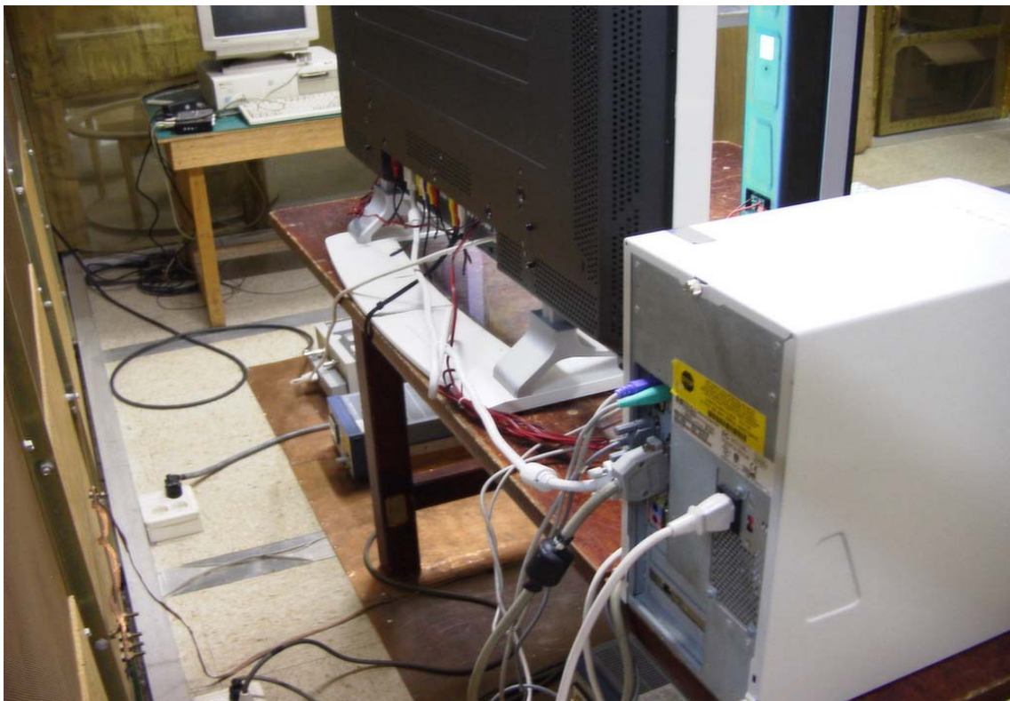
Conducted Emission 450kHz ~ 30MHz Mode : Scrolling “H” Pattern
