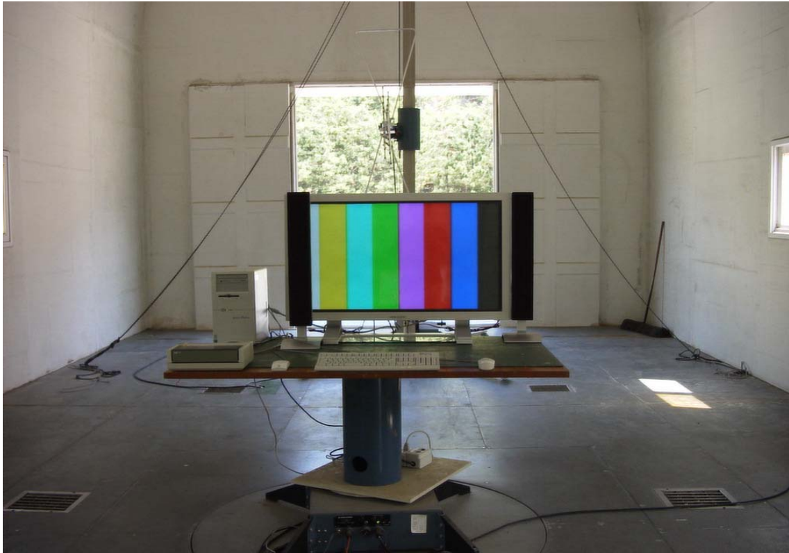
Radiated Emission 30MHz ~ 1000MHz Mode : Color bar
