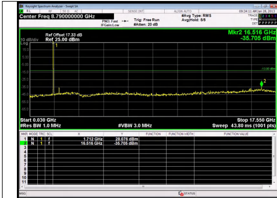
30.0MHz-17550.0MHz Band 4 20MHz/1720.0/Low QPSK 1@0
