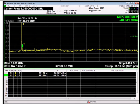
30.0MHz-8490.0MHz Band 5 1.4MHz/848.3/High 16QAM 1@0
