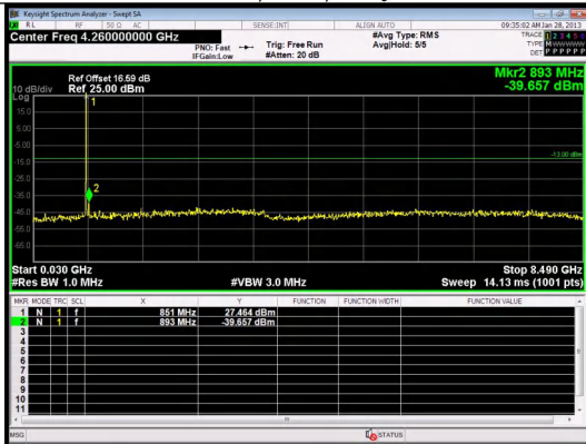
30.0MHz-8490.0MHz Band 5 1.4MHz/848.3/High QPSK 1@0
