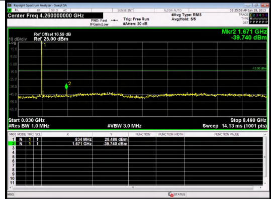
30.0MHz-8490.0MHz Band 5 1.4MHz/836.5/Mid 16QAM 1@0
