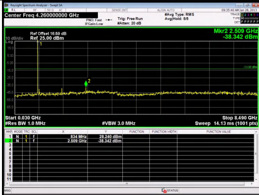
30.0MHz-8490.0MHz Band 5 1.4MHz/836.5/Mid QPSK 1@0
