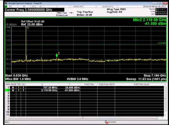
30.0MHz-7160.0MHz Band 12 3MHz/707.5/Mid 16QAM 1@0
