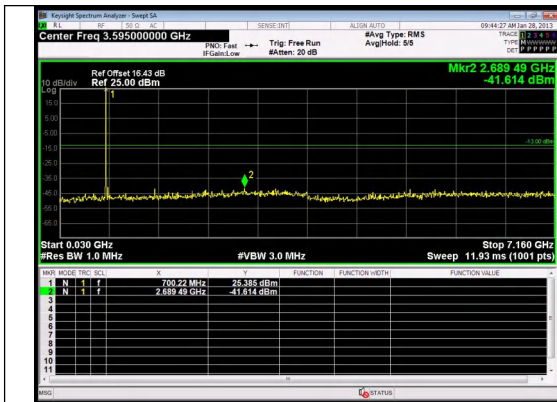
30.0MHz-7160.0MHz Band 12 1.4MHz/699.7/Low QPSK 1@0
