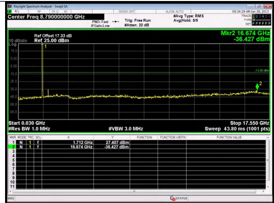
30.0MHz-17550.0MHz Band 4 20MHz/1720.0/Low 16QAM 1@0
