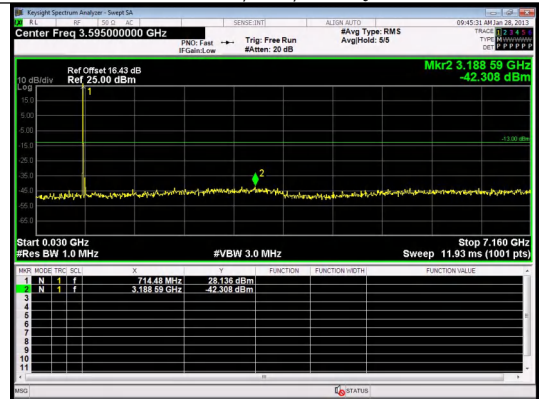
30.0MHz-7160.0MHz Band 12 3MHz/714.5/High 16QAM 1@0
