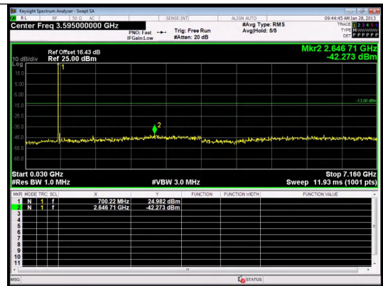
30.0MHz-7160.0MHz Band 12 1.4MHz/699.7/Low 16QAM 1@0
