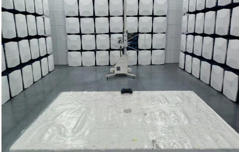
Radiated Emission
