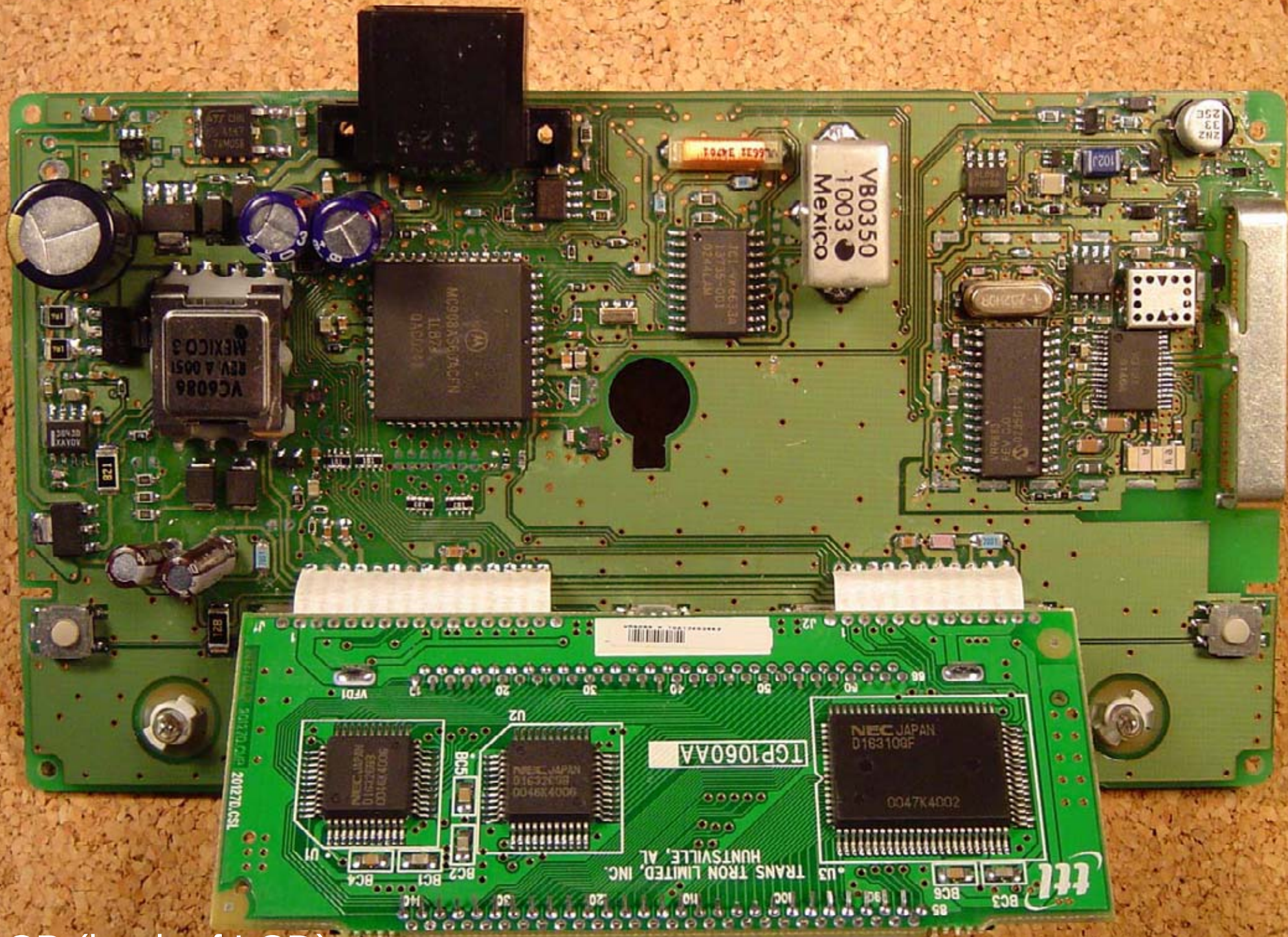
PCB (back of LCD)
