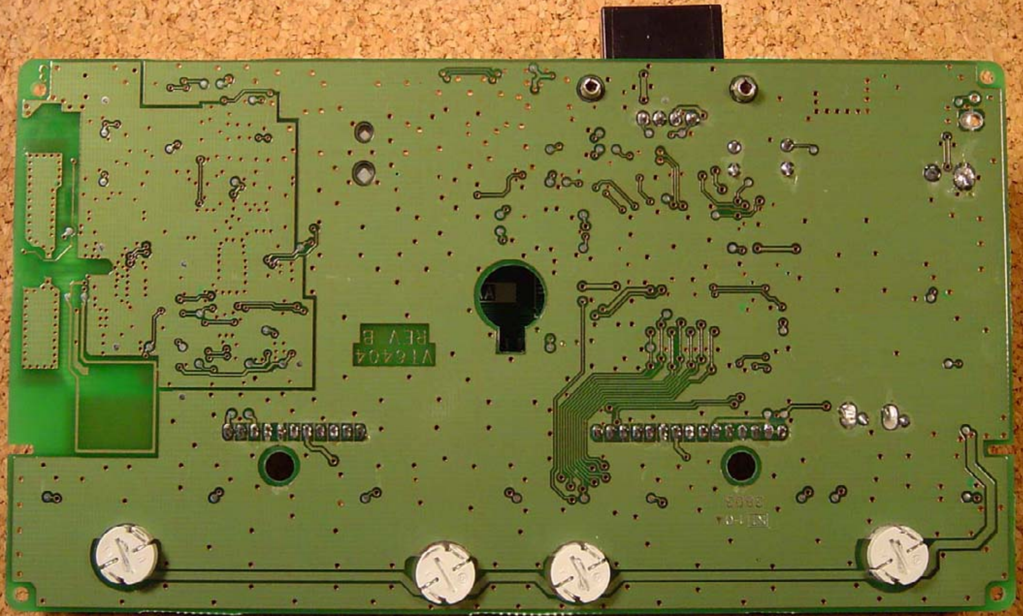
PCB (bottom)
