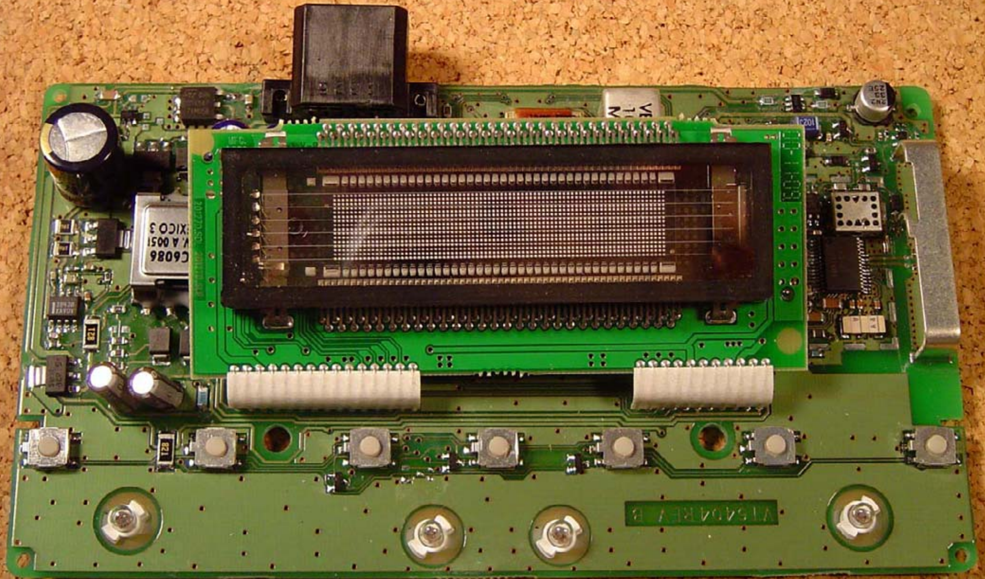
PCB (top)
