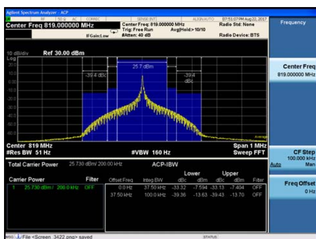
NB-IOT Band 26 BPSK 3.75kHz 1@47 CH-High
