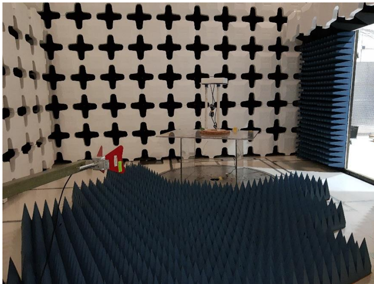
Figure 2.REE Test Setup above 1GHz
